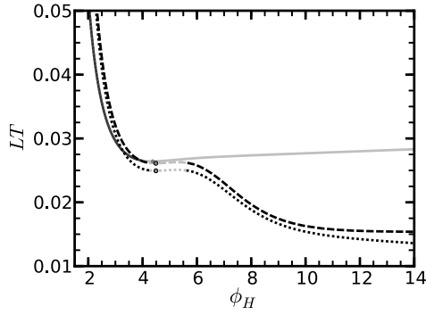
Fig. A.3. The temperature as a function of \phi_H for the potentials v_1 (8) with parameters (10) (solid curve) as well as v_{2a} (dashed curve) and v_{2b} (dotted curve), see (A.1) and (A.2). Light grey portions of the curves denote the unstable/metastable regions of the equation of state, while dots mark the positions of \phi_H^{\min} .
