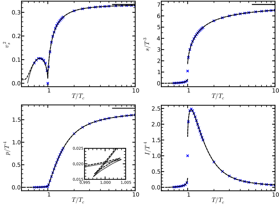
Fig. A.1. The same as Fig. 1 but extending the lattice data points and model calculation into the confined phase for the potential v_2 (A.1) with parameters (A.2). Solid curves: v_{2a} , dashed curves: v_{2b} . The unstable/metastable branches are not plotted, unless in the inset of the pressure panel, where the standard loop structure is displayed for p/T^4 with p calculated from (9).
