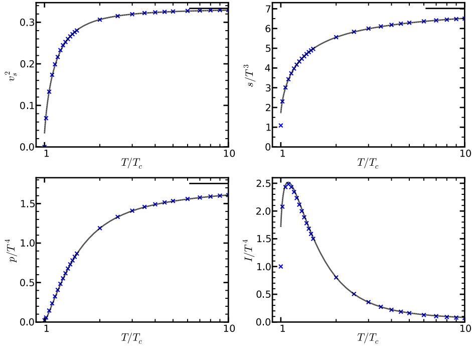
Fig. 1. The sound velocity squared v_s^2 (left top panel), scaled entropy density s/T^3 (right top panel), scaled pressure p/T^4 (left bottom panel), and scaled interaction measure I/T^4 (right bottom panel) as functions of T/T_c for the potential v_1 (8) with optimized parameters (10). The lattice data (symbols) are from [1]. The horizontal lines in the upper right corners depict the respective Stefan-Boltzmann limits.
