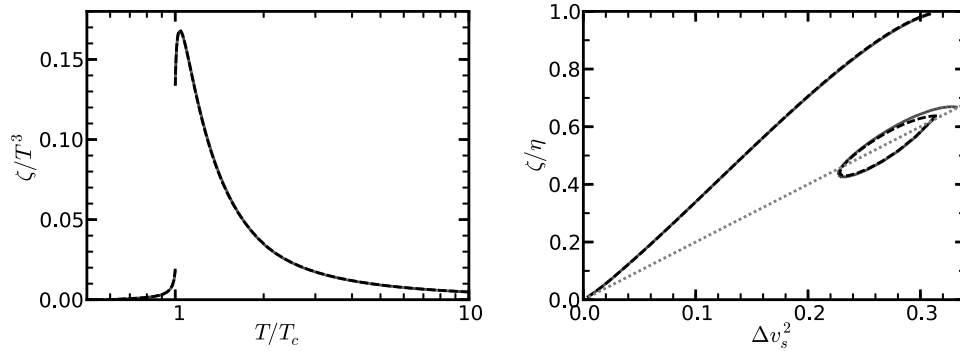
Fig. A.2. The scaled bulk viscosity \zeta/T^3 as a function of the temperature (left panel) and the ratio \zeta/\eta as a function of the non-conformality measure (right panel). Line codes are the same as in Fig. A.1. The grey dotted line in the right panel depicts the Buchel bound.
