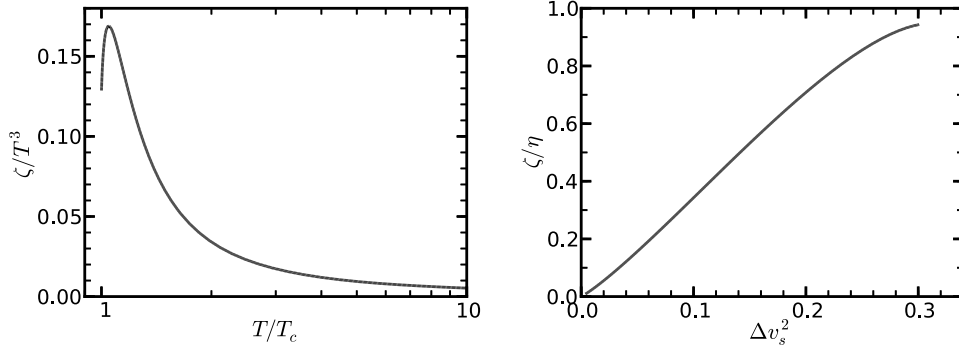
Fig. 2. The scaled bulk viscosity \zeta/T^3 as a function of the temperature (left panel) and the ratio \zeta/\eta as a function of the non-conformality measure (right panel).
