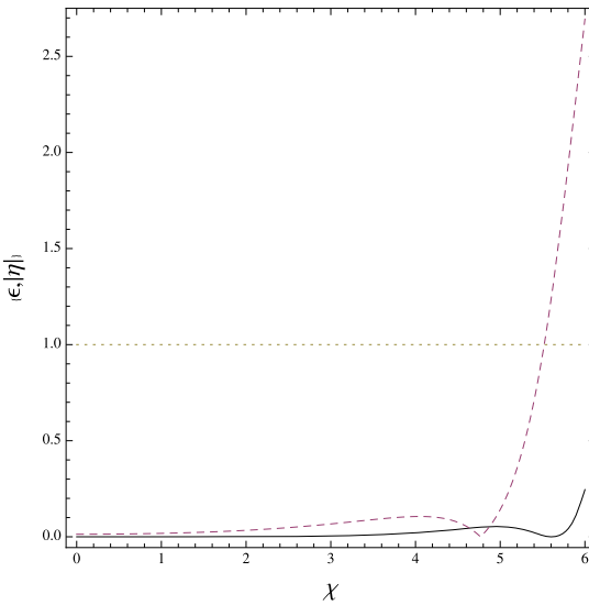
Fig. 2. Behavior of the slow-roll parameters. The parameters are chosen to be same as in Fig. 1. The dashed line is for \eta and the solid line is for \epsilon .
