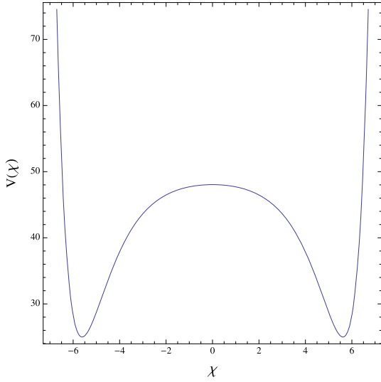
Fig. 1. Behavior of the potential for B = -0.96 , K = 1 . A and V_1 are chosen to be -1 and 49 in units of \frac{\kappa^2 M_{pl}^2}{2} . Here \chi is shown in units of M_{pl} and V(\chi) in units of M_{pl}^4 .
