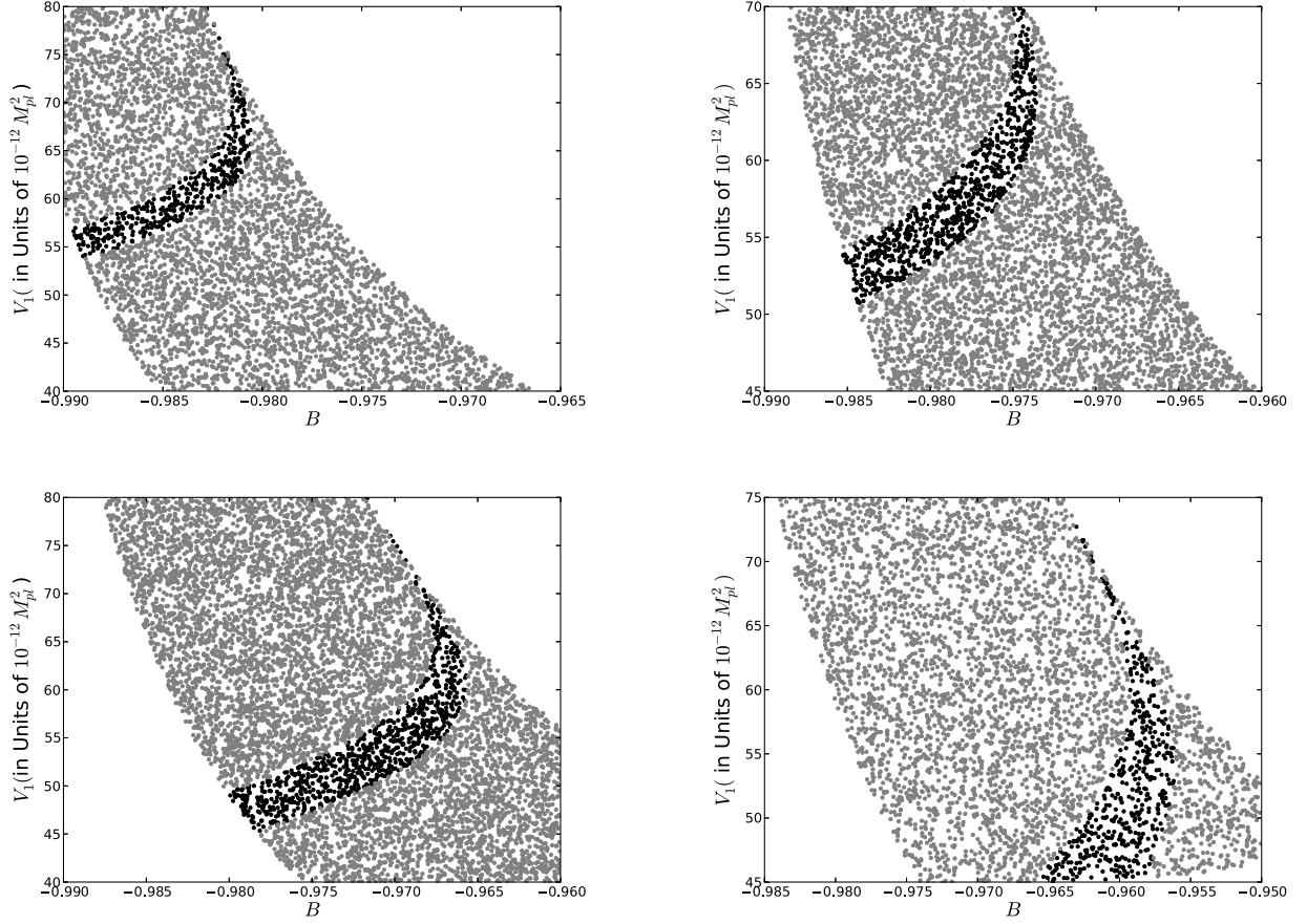
Fig. 3. The allowed region in B - V_1 plane for K = 1 . Grey dots represent the points for which inflation successfully happens but do not satisfy Planck constraints. Black dots do satisfy Planck constraints given in Eq. (32). Values of A are A = -0.6 \times 10^{-12} M_{pl}^2 (top left), -0.8 \times 10^{-12} M_{pl}^2 (top right), -1.0 \times 10^{-12} M_{pl}^2 (bottom left) and -1.2 \times 10^{-12} (bottom right).
