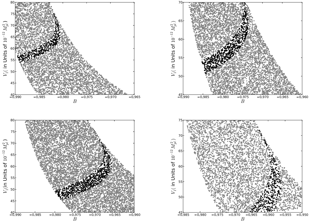
Fig. 3. The allowed region in B - V_1 plane for K = 1 . Grey dots represents the points for which inflation successfully happens but do not satisfy Planck constraints. Black dots do satisfy Planck constraints given in Eq. (32). Values of A are A = -0.6 \times 10^{-12} M_{pl}^2 (top left), -0.8 \times 10^{-12} M_{pl}^2 (top right), -1.0 \times 10^{-12} M_{pl}^2 (bottom left) and -1.2 \times 10^{-12} (bottom right).
