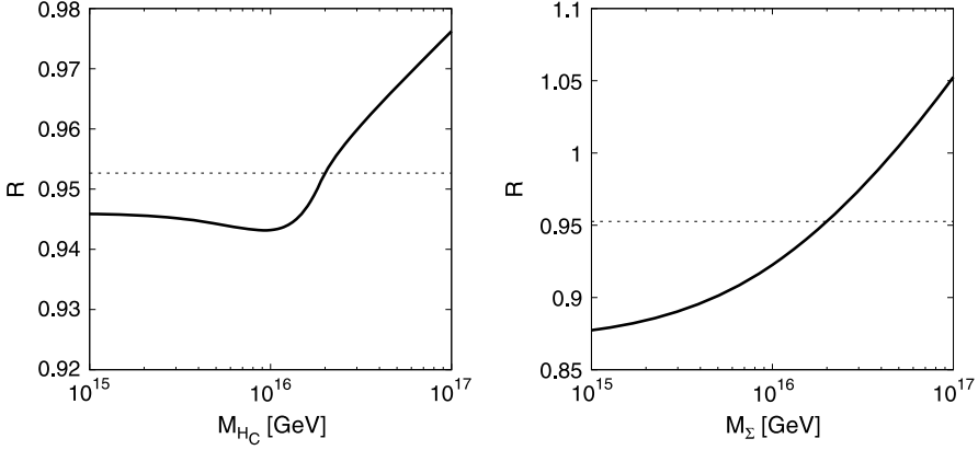
Fig. 6. GUT-scale particle mass dependence on renormalization factor of proton decay. Left panel shows M_{H_C} dependence for M_\Sigma = M_X = 2 \times 10^{16} GeV. Right panel shows M_\Sigma dependence for M_{H_C} = M_X = 2 \times 10^{16} GeV. Dotted line shows the degenerate mass case in each panels.
