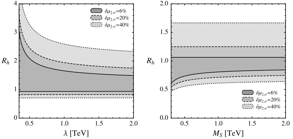
Fig. 6. Combined 2\sigma LEP and future LHC WBF (or current all-channels) constraints on the Higgs width in the model with modified couplings and a UV cutoff (left) and a model with a mixed-in singlet scalar (right).
