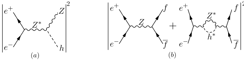
Fig. 1. (a) The dominant Higgs production process at a potential future Higgs factory e^+e^- collider and (b) Z-boson production and decay at an e^+e^- collider including interference of one loop diagrams involving an off-shell Higgs. An analogy between the on-shell and off-shell Higgs factory is drawn because the squared amplitude for the Higgs factory is related to the one-loop amplitude which interferes with tree-level diagrams at an off-shell Higgs factory.
