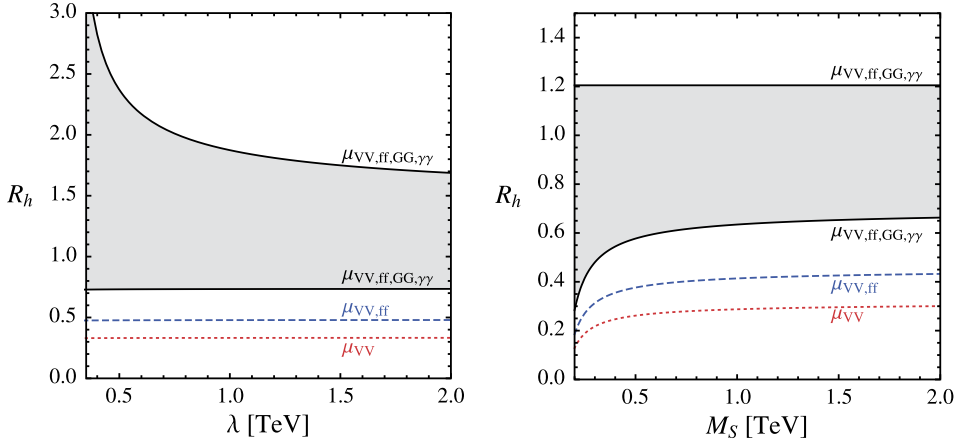
Fig. 5. Combined 2\sigma LEP and current LHC signal strength constraints on the Higgs width in the model with modified couplings and a UV cutoff (left) and a model with a mixed-in singlet scalar (right). Please see the surrounding text for an explanation of the various contours.
