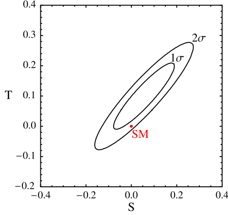
Fig. 3. The standard S – T ellipse for U = 0 with the SM point depicted at S = T = 0 .
