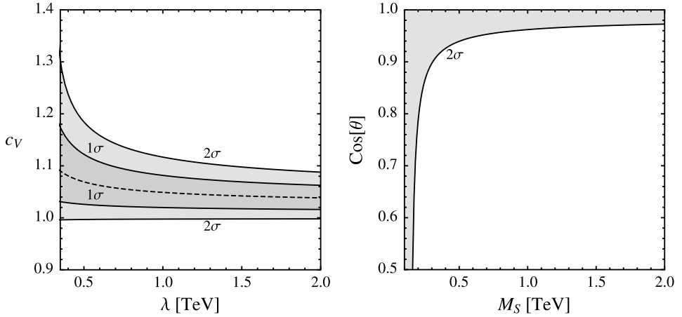
Fig. 4. LEP constraints on modified Higgs couplings in the two models described in Sec. 2. There is already tension at 1\sigma between precision electroweak fits and the SM, hence in the models model with re-scaled couplings (left panel) the SM limit is only within the 2\sigma contours. For the Higgs portal model (right panel) we only show the 2\sigma contour.
