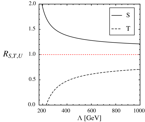
Fig. 2. The ratio of full loop functions in Eq. (8) with the leading-log expressions in Eq. (9) as a function of the UV cutoff \Lambda . It is clear that the leading-log expressions may underestimate ( S ) or overestimate ( T ) the corrections by more than 20%, even with a cutoff extending to 1 TeV where one might expect the leading-log expression to be accurate. However, the leading-log result is often adequate for estimates as it is the dominant contribution for \Lambda \gtrsim 300 GeV.
