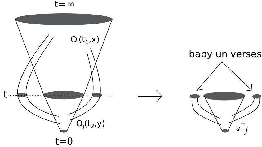
Fig. 1. Universe and baby universes. Here, we show wormholes having two legs. The left and right figures represent the partition function and Hamiltonian points of view respectively.
