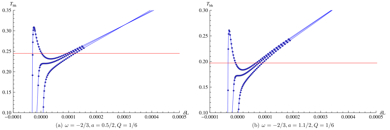
Fig. 5. Relations between the two point correlation function and temperature for different a with a fixed \omega = -2/3 . The red solid lines correspond to the locations of first order phase transition.
