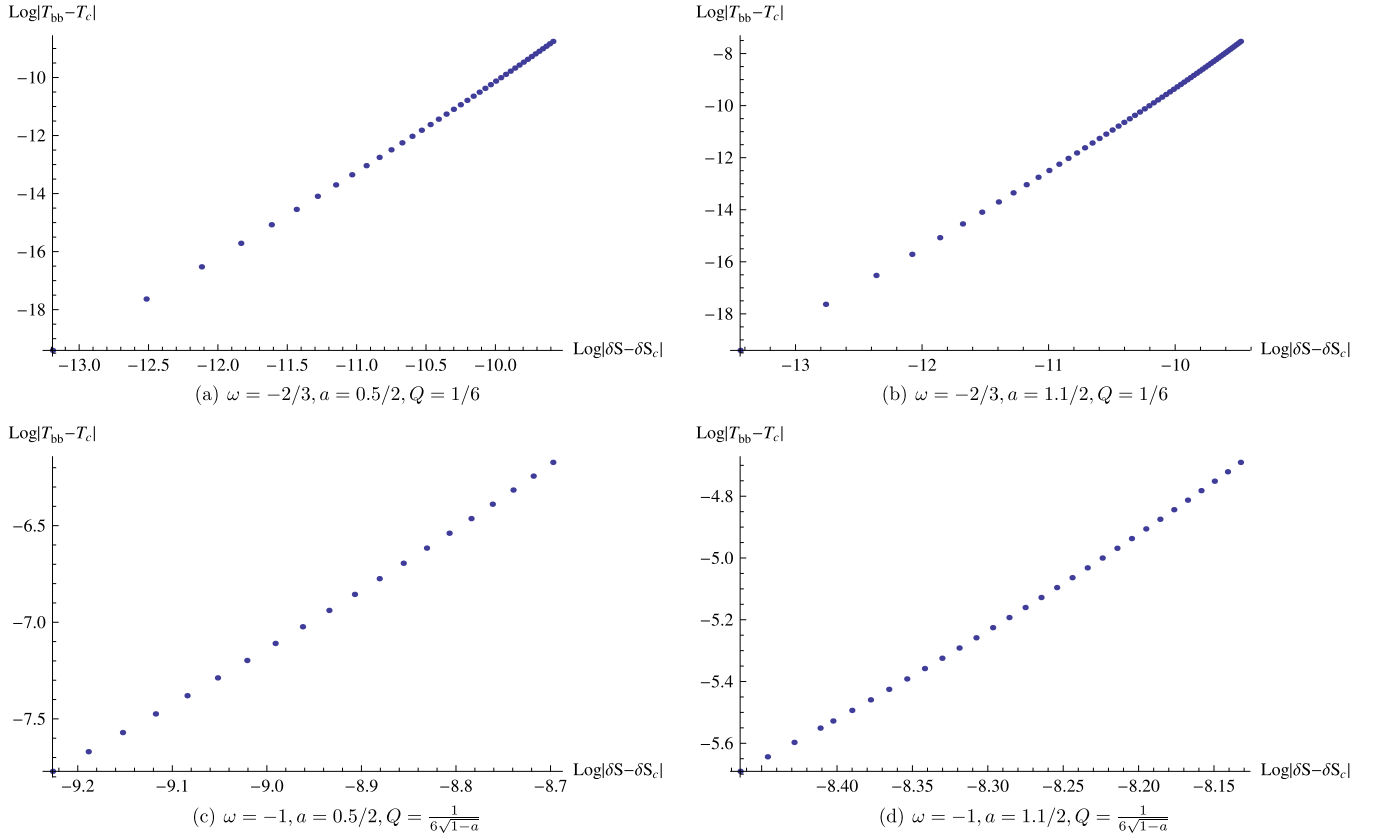
Fig. 4. Relations between \log |T_{bh} - T_c| and \log |\delta S - \delta S_c| for different \omega and a .
