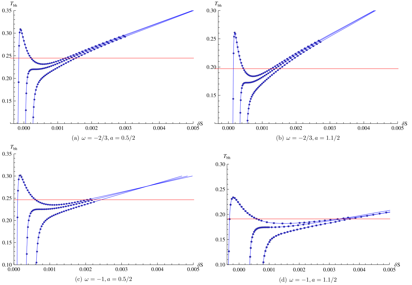
Fig. 3. Relations between the entanglement entropy and temperature for different \omega and a . The red solid lines correspond to the locations of first order phase transition.
