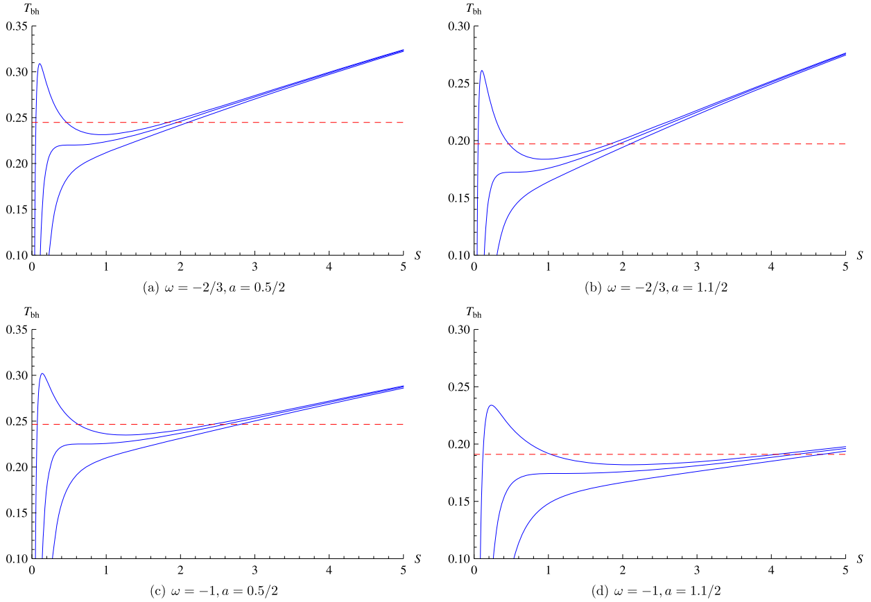
Fig. 1. Relations between the entropy and temperature for different \omega and a . The red dashed lines correspond to the locations of first order phase transition.
