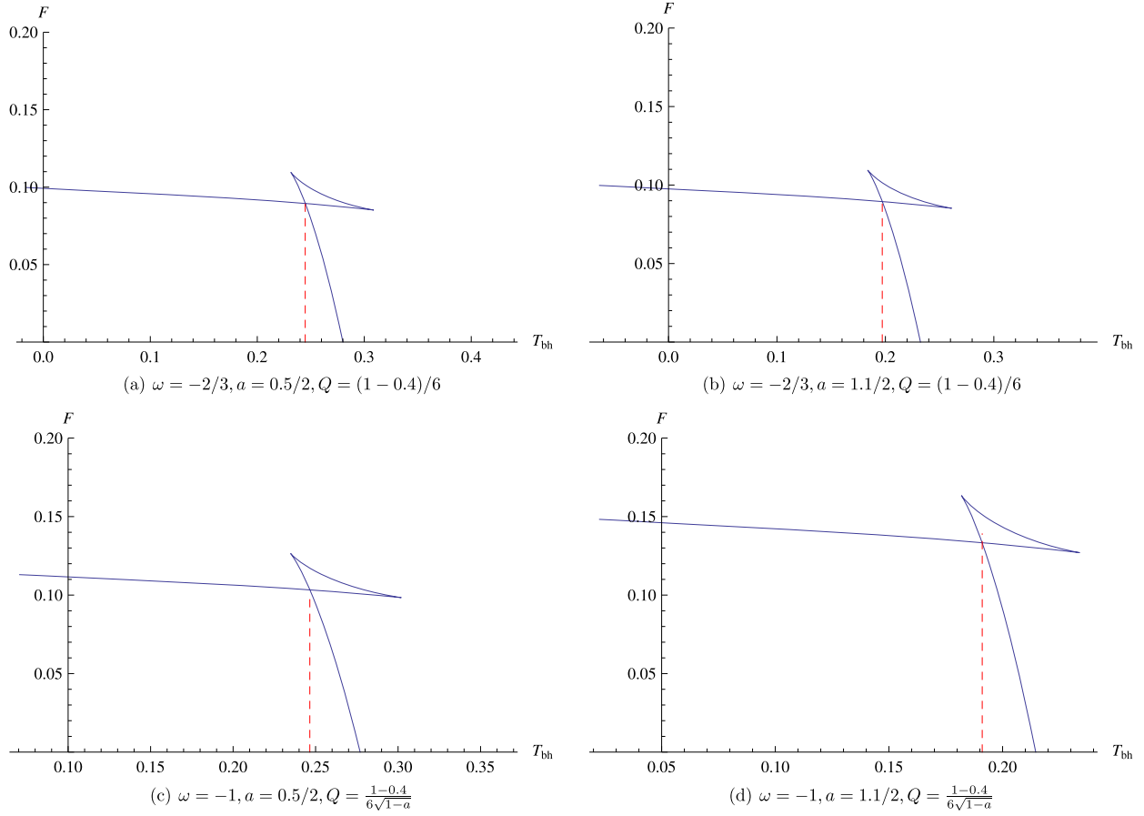
Fig. 2. Relations between the free energy and temperature for different \omega and a . The intersection point between the red dashed line and horizontal coordinate in each graph is the first order phase transition temperature.
