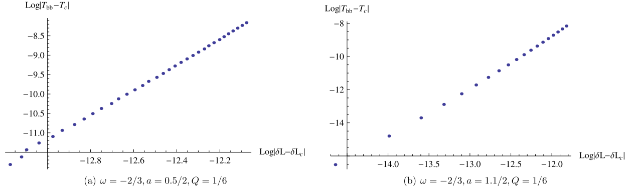
Fig. 6. Relations between \log |T_{bh} - T_c| and \log |\delta L - \delta L_c| for different a .
