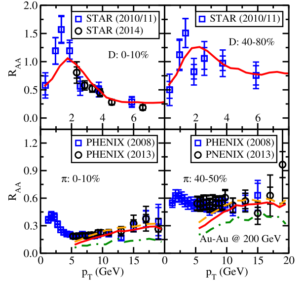
Fig. 2. (Color online.) Nuclear suppression factor R_{AA} of D and \pi spectra in 200 AGeV Au–Au collisions at RHIC. Data are taken from Refs. [44,54,55]. Contributions to \pi spectra from quarks (upper curves with dashed lines), gluons (lower curves with dot-dashed lines) and the sum of them (middle curves with solid lines) are shown separately in the lower panels.
