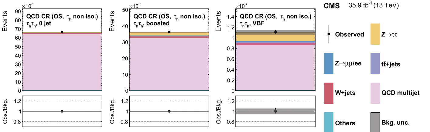
Fig. 4. Control regions enriched in the QCD multijet background used in the maximum likelihood fit, together with the signal regions, to extract the results. The normalization of the predicted background distributions corresponds to the result of the global fit. These regions, formed by selecting events with opposite-sign \tau_h candidates passing relaxed isolation requirements, control the yields of the QCD multijet background in the \tau_h\tau_h channel.
