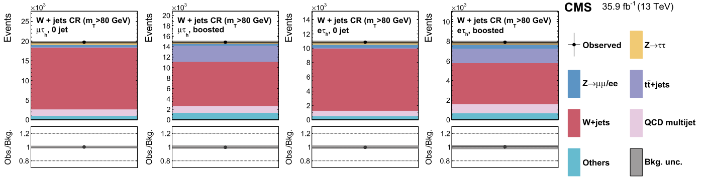
Fig. 2. Control regions enriched in the W + jets background used in the maximum likelihood fit, together with the signal regions, to extract the results. The normalization of the predicted background distributions corresponds to the result of the global fit. These regions, defined with m_T > 80 GeV, control the yields of the W + jets background in the \mu\tau_h and e\tau_h channels. The constraints obtained in the boosted categories are propagated to the VBF categories of the corresponding channels.
