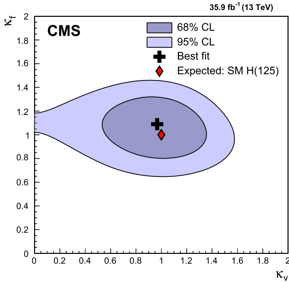
Fig. 22. Scan of the negative log-likelihood difference as a function of \kappa_V and \kappa_F , for m_H = 125.09 GeV. All nuisance parameters are profiled for each point. For this scan, the pp \rightarrow H \rightarrow WW contribution is treated as a signal process.
