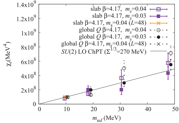
Fig. 5. m_{ud} dependence of topological susceptibility at \beta = 4.17 obtained from \langle Q_{\text{slab}}^2(T_{\text{cut}}) \rangle (solid symbols) and those from the global topological charge (dashed, slightly shifted to avoid overlapping with the former data). The LO prediction from SU(2) ChPT, where the chiral condensate \Sigma^{1/3} = 270 \text{ MeV} , is also shown to guide the eye.
