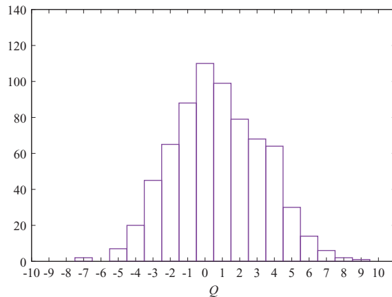
Fig. 1. The distribution of \sum_x q^{\text{lat}}(x) at \beta = 4.17 , m_{ud} = 0.007 , and m_s = 0.04 .
