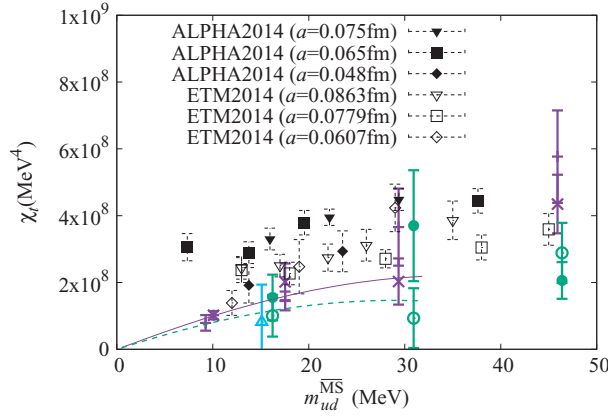
Fig. 8. The same figure as Fig. 7 but a comparison with Ref. [8] (ETM2014, N_f = 2 + 1 + 1 results converted using the input r_0 = 0.46 fm) and Ref. [9] (ALPHA2014, N_f = 2 results converted assuming m_{ud} = M_\pi^2 F_\pi^2 / (2\Sigma) using the inputs t_1 = 0.061 fm 2 , F_\pi = 92 MeV, and \Sigma = (270 \text{ MeV})^3 ) is shown.
