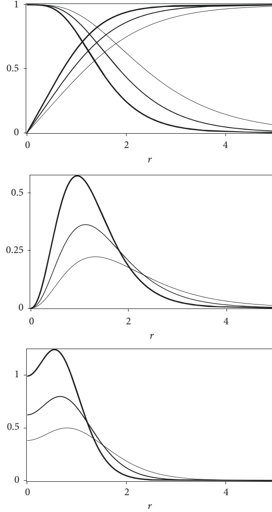
FIGURE 3: The solutions a(r) (descending lines) and g(r) (ascending lines) of (30a) and (30b) (top), the magnetic field (middle), and the energy density (bottom) of the visible sector for q, w = 1 and \beta = 0.5, 1 and 2 . The thickness of the lines increases with \beta .
