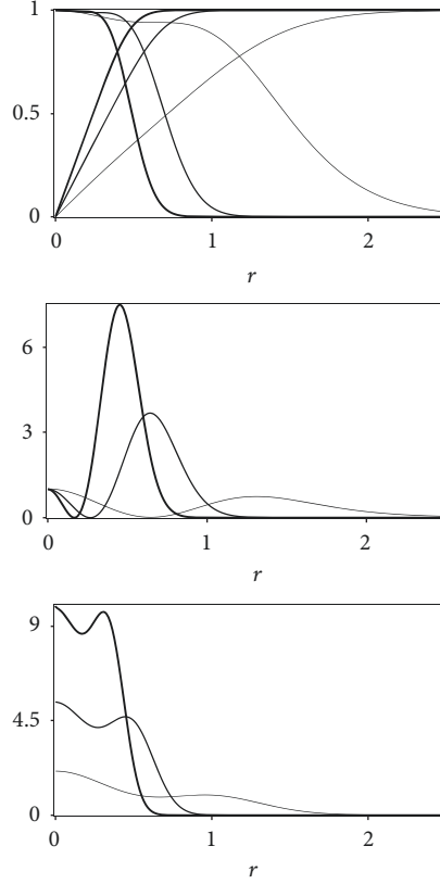
FIGURE 1: The solutions a(r) (descending lines) and g(r) (ascending lines) of (22a) and (22b) (top), the magnetic field (middle), and the energy density (bottom) of the visible sector for q, w = 1 and \beta = 4, 20 and 50 . The thickness of the lines increases with \beta .
