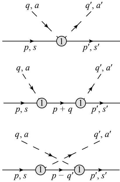
Fig. A1. The tree diagrams at O(p^1) level.
