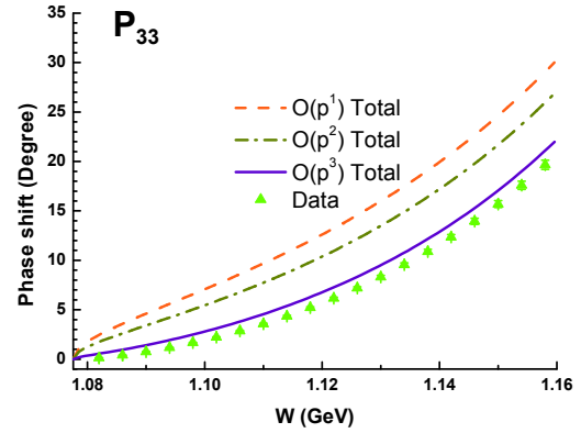
Fig. 12. (color online) PKU-representation analysis of P_{33} channel. (left) known contributions vs the data. (right) known contributions with l.h.c.s estimated in different chiral orders ( s_c = -0.08 \text{ GeV}^2 ).
