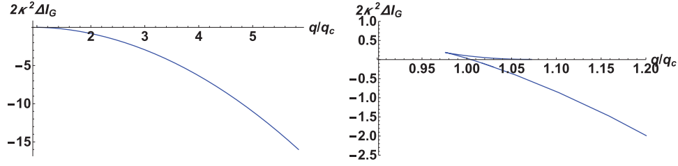
Fig. A.2. The difference in the normalized free energy 2\kappa^2\Delta I_G is plotted at fixed temperature T_H = 0.15 . Left: Fixed \tilde{\kappa}^2 = 0.1 . It shows that, at large charge density q > q_c (= 33.5T_H = 5.02) , the condensed phase is favored. Right: Fixed \tilde{\kappa}^2 = 0.5 . There is the swallow tail of the first-order phase transition at the critical charge density q = q_c (= 189T_H = 28.3) .
