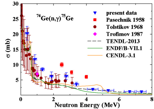
Fig. 5. (Color online.) ^{74}\text{Ge}(n, \gamma)^{75}\text{Ge} total cross-section data in comparison to the previously existing data and evaluations and the model prediction TENDL-2013. The ENDF/B-VII.1 and JENDL-4.0 [28] evaluations overlap in the entire energy range.
