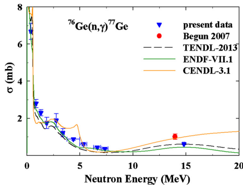
Fig. 3. (Color online.) ^{76}\text{Ge}(n, \gamma)^{77}\text{Ge} total cross-section data in comparison to evaluations and the model prediction TENDL-2013. The ENDF/B-VII.1 and JENDL-4.0 [28] evaluations overlap in the entire energy range. The datum of Begun et al. [26] is the only cross-section value that existed before the present measurements.
