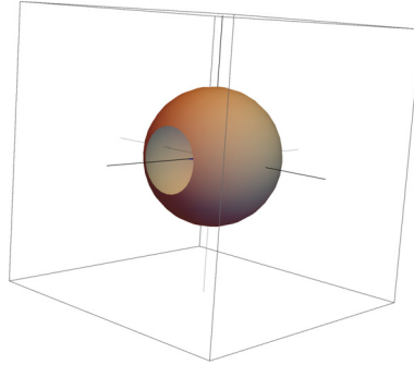
Fig. 5. (Color online.) Applying the transverse field of Eq. (8) to the ring of Fig. 4 leads to precession about the S_{tot}^y axis. For the above displayed ring, \theta(t) = \pi/2 . During the precession, the semi-classical total spin vectors \vec{S}_{tot} on the ring acquire a range of possible S_{tot}^z values leading to the standard deviation \sigma_\epsilon of the energy density of Eq. (6). The simple (semi-classical) calculation of Eq. (16) for the distribution of S_{tot}^z values for such a uniform ring leads anew to Eq. (13).
