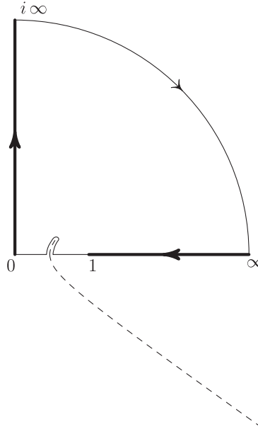
Fig. 2. Location of the relevant discontinuity cut \mathcal{C}_{ij} with respect to the two half straight lines [0, +i\infty[ and [1, +\infty[ , and deformation of the contour \widehat{(0, 1)} partly wrapping the extremity of the cut.
