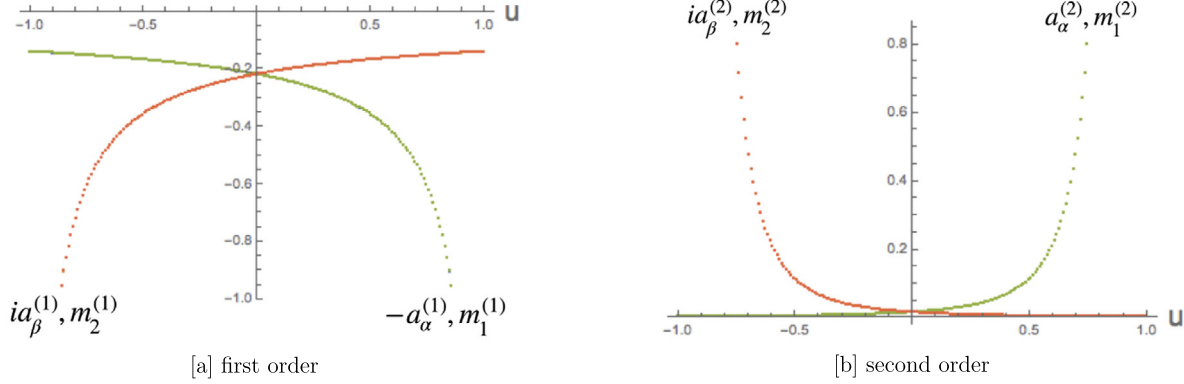
Fig. 3.2. The numerical results of [a] the first order and [b] the second order ( \Lambda = 1 , u = -0.6 ). The green lines show the results of (-1)^n a_\alpha^{(n)}, m_1^{(n)} and the red lines show the results of ia_\beta^{(n)}, m_2^{(n)} .
