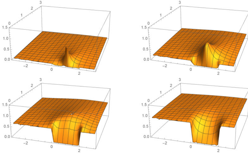
Fig. 6. Profiles of the fidelity A_{n=1/2, m=1/2} = \text{Tr}[\sqrt{\sqrt{\rho}\rho'\sqrt{\rho}}] in c = 1 free scalar CFT for the operator O = e^{i\phi} , which has the dimension h = 1/2 when we change the value of w . The upper left, upper right, lower left, and lower right graphs describe A_{n=1/2, m=1/2} for w = 1 + 0.05i , w = 1 + 0.2i , w = 1 + 0.8i , and w = 1 + 2i , respectively. A_{n=1/2, m=1/2} is plotted as a function of (p, q) for \rho'(w' = p + iq) , with L = 2 .
