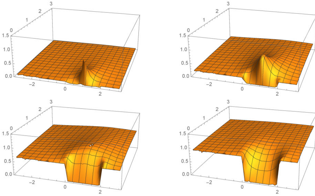
Fig. 6. Profiles of the fidelity A_{n=1/2, m=1/2} = \text{Tr}[\sqrt{\sqrt{\rho}\rho'\sqrt{\rho}}] in c = 1 free scalar CFT for the operator O = e^{i\phi} , which has the dimension h = 1/2 when we change the value of w . The upper left, upper right, lower left, and lower right graphs describe A_{n=1/2, m=1/2} for w = 1 + 0.05i , w = 1 + 0.2i , w = 1 + 0.8i , and w = 1 + 2i , respectively. A_{n=1/2, m=1/2} is plotted as a function of (p, q) for \rho'(w' = p + iq) , with L = 2 .
