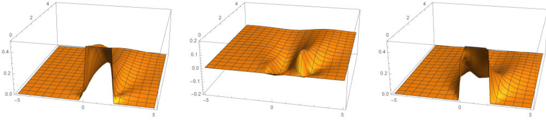
Fig. 7. Profiles of the Bures metric for c = 1 free scalar CFT as a function of w = x + i\tau : \tau^2 G_{\tau\tau} (left), \tau^2 G_{\tau x} (middle), and \tau^2 G_{xx} (right) as functions of x and \tau , with L = 2 . At the boundary \tau \rightarrow 0 , we find \tau^2 G_{\tau\tau, xx} \rightarrow \frac{1}{2} and \tau^2 G_{\tau x} \rightarrow 0 .
