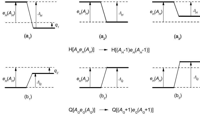
Fig. 1. Schematic diagrams of nuclear levels when hadronic matter losses a nucleon and hence quark matter captures a nucleon. Panels (a 1 ) and (b 1 ) represent the case of release binding energies.
