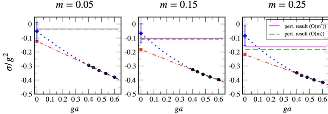
Fig. 4. Continuum extrapolations of the string tensions \sigma/g^2 in the charge-3 Schwinger model for q_p = -1 and \theta_0 = 2\pi at the physical volume ga(N-1) = 9.6 . The linear and quadratic fits in terms of ga are considered (shown with red dot-dashed lines and blue dotted curves, respectively). The theoretical predictions in the continuum limit are based on the first- (green dashed line) and second- (magenta solid line) order approximations of the mass perturbation theory. The error bars associated with the black circles denote the fitting errors in finding the string tensions from Fig. 3.
