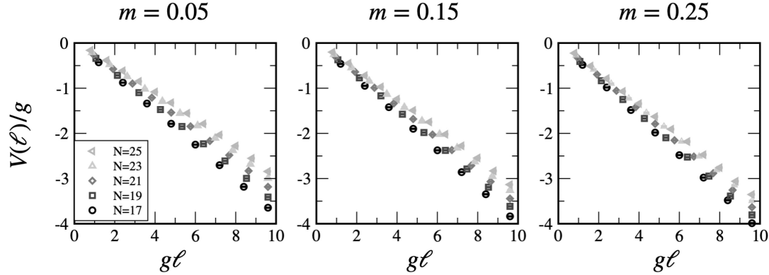
Fig. 3. The potentials V(\ell)/g in the charge-3 Schwinger model for q_p = -1 and \theta_0 = 2\pi are plotted for various values of (a, N) with a fixed physical volume ( ga(N-1) = 9.6 ).
