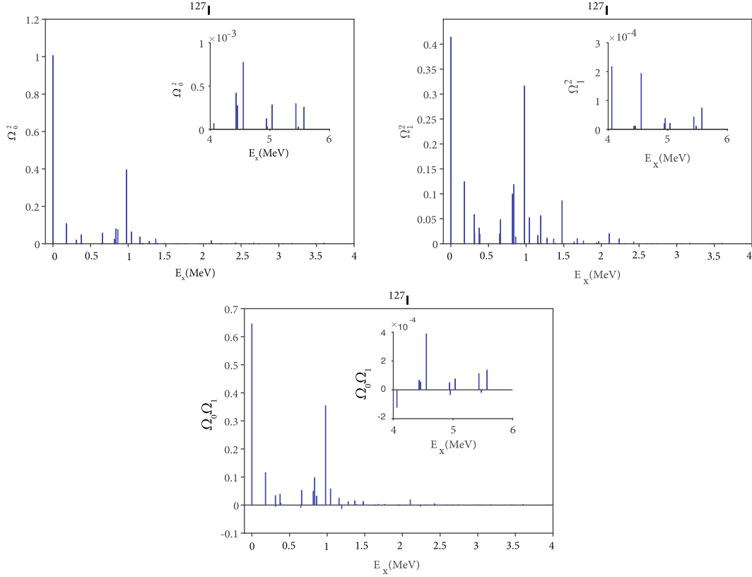
FIGURE 5: Isoscalar and isovector spin matrix elements up to 6 MeV relevant for axion absorption are presented. Note that in the range of 4–6 MeV, in order to make the matrix elements visible, we exhibit them in a separate small window, where the small scale is indicated.
