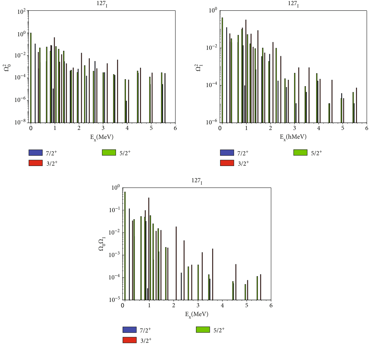
FIGURE 4: Isoscalar and isovector distribution of ^{127}\text{I} spin-reduced matrix elements from J_i = 5/2^+_{\text{gs}} to J_f relevant for axion photoproduction. We should mention that the energy of the emitted photon is E_\gamma = E_a - E_x ; i.e., the maximum photon energy corresponds to the gs to gs transition.
