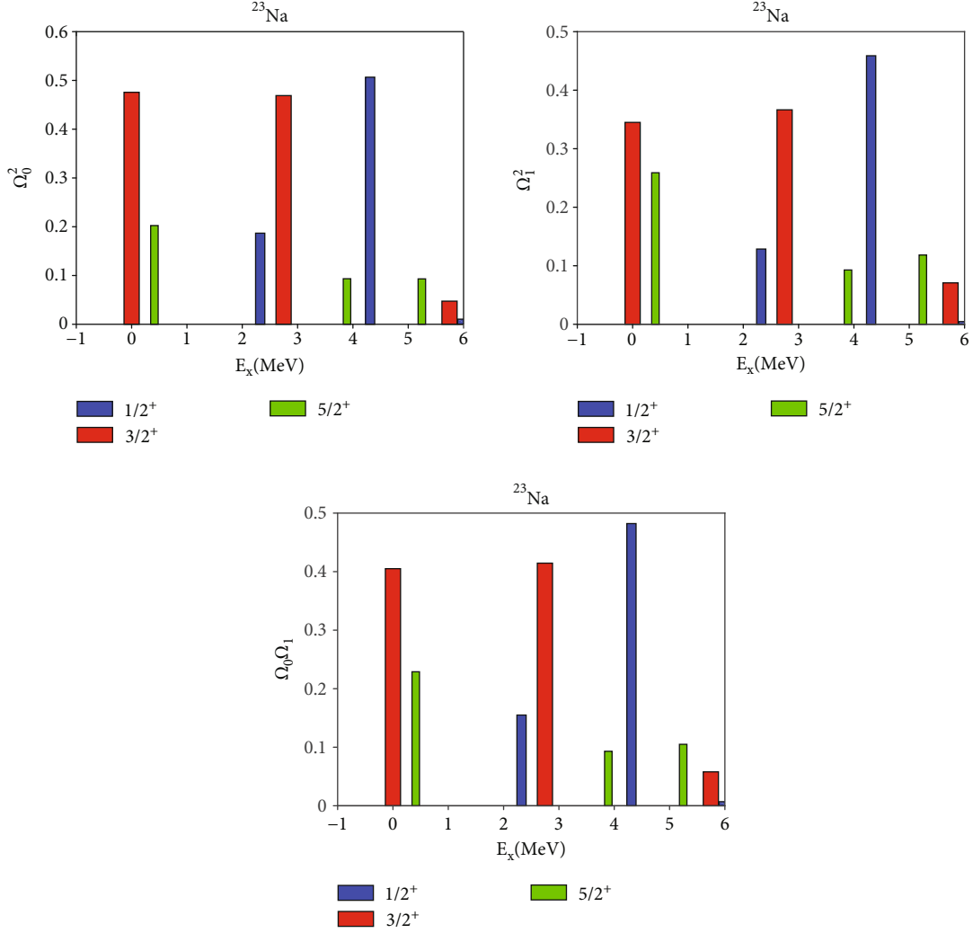
FIGURE 6: Isoscalar and isovector distribution of ^{23}\text{Na} spin-reduced matrix elements from J_i = 3/2^+ to J_f relevant for axion photoproduction. We should mention that the energy of the emitted photon is E_\gamma = E_a - E_x ; i.e., the maximum photon energy corresponds to the gs to gs transition.
