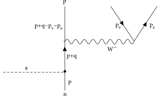
FIGURE 2: A Feynman diagram relevant for axion-induced beta decay.
