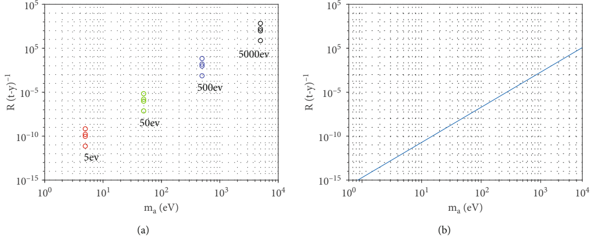
FIGURE 7: (a) Event rates for the last four states 4.31 MeV, 5.24 MeV, 5.74 MeV, and 5.97 MeV of ^{23}\text{Na} (see Table 2) versus different axion masses. (b) The rate for axion photoproduction on ^{127}\text{I} . As expected, this is quite a bit smaller than in (a), due to the fact that the axion energy of 5.5 MeV is much smaller than the nucleon mass. Note, however, that in this case, we have the extra signature of the produced photon. Since the rate is dominated by the coherent mode, the photon energy is approximately equal to the axion energy.
