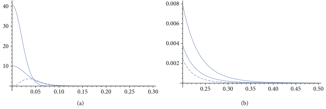
FIGURE 8: (a) We exhibit the dependence of the form factors encountered in the ionization of Na as a function of the momentum transfer, here momentum of the emitted electron p_e in units of the electron mass. (b) The same figure restricted to higher momentum transfers. The solid line corresponds to n=1 , the thick solid line to n=2, \ell=0 , and the dashed line to n=2, \ell=1 .
