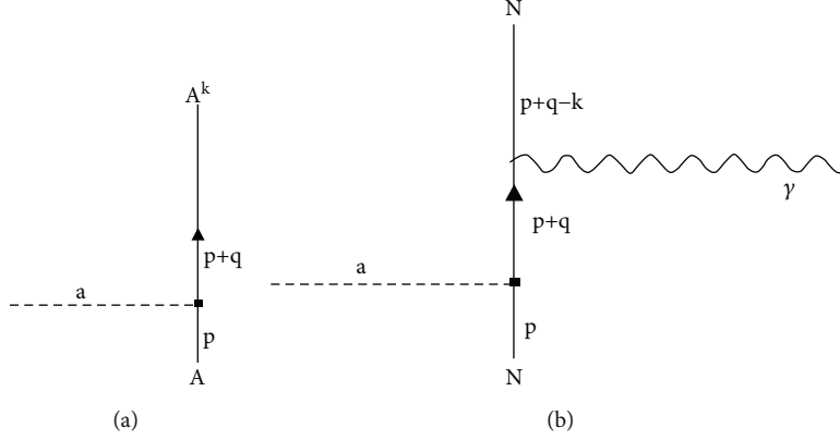
FIGURE 1: (a) An axion is absorbed by a nucleus leading to an excited nuclear state. (b) A Feynman diagram relevant for axion photoproduction. In both cases, in the axion vertex, we encounter the coupling given by Equation (17), while in the EM vertex in (b), we have the usual interaction involving the nuclear magnetic moment. p , q , and k are the initial nucleon, axion, and photon 4-momenta, respectively. In both cases of (a) and (b), the output signal energies are the same, 5.5 MeV.
