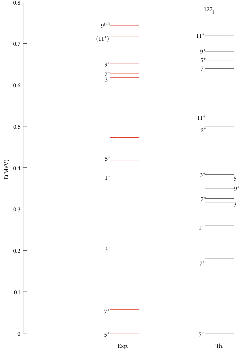
FIGURE 3: The low-lying experimental (a) [62] and theoretical (b) energy spectrum of ^{127}\text{I} . The levels in the figure are labeled by 2J . Note that the spin and parity of the experimental states at 0.295 MeV and 0.473 MeV are not known.
