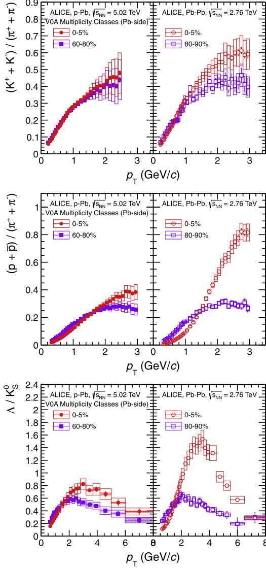
Fig. 2. (Color online.) Ratios K/\pi = (K^+ + K^-)/(\pi^+ + \pi^-) , p/\pi = (p + \bar{p})/(\pi^+ + \pi^-) and \Lambda/K_S^0 as a function of p_T in two multiplicity bins measured in the rapidity interval 0 < y_{\text{CMS}} < 0.5 (left panels). The ratios are compared to results in Pb-Pb collisions measured at mid-rapidity, shown in the right panels. The empty boxes show the total systematic uncertainty; the shaded boxes indicate the contribution uncorrelated across multiplicity bins (not estimated in Pb-Pb).
