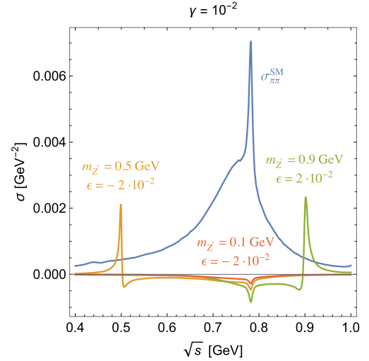
Fig. 3. \sigma_{\pi\pi}^{\text{SM}} and \Delta\sigma_{\pi\pi}^{\text{NP}} for some benchmark values of the Z' model parameters solving the \Delta a_\mu discrepancy, see Eq. (1).
