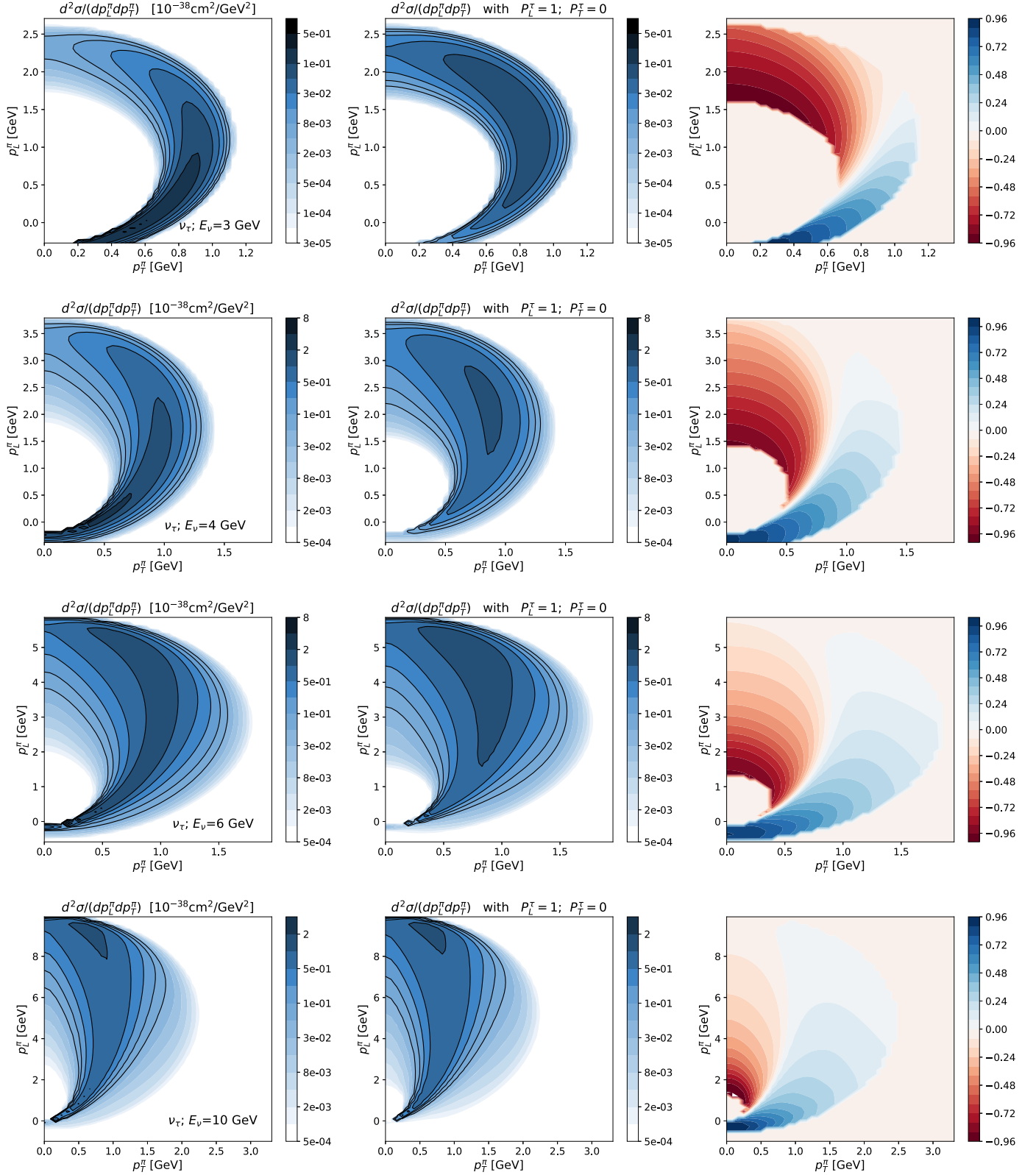
Fig. 2. Two-dimensional d^2\sigma/(dp_L^\tau dp_T^\pi) distributions, in units of 10^{-38} \text{ cm}^2/\text{GeV}^2 , for the sequential \nu_\tau A_Z \rightarrow \tau^-(\pi^-\nu_\tau)X process evaluated in ^{16}\text{O} at E_\nu = 3, 4, 6 and 10 GeV (shown from top to bottom). The left panels show the full calculation of Eqs. (16). In the middle panels we set P_L^\tau = 1, P_T^\tau = 0 , which corresponds in our case to pure negative-helicity taus. Finally, the right panels show the ratio of the difference of the two previous calculations over their sum. We consider only the QE contribution computed using the LFG model of Ref. [11], without including RPA and correct-energy balance corrections.
