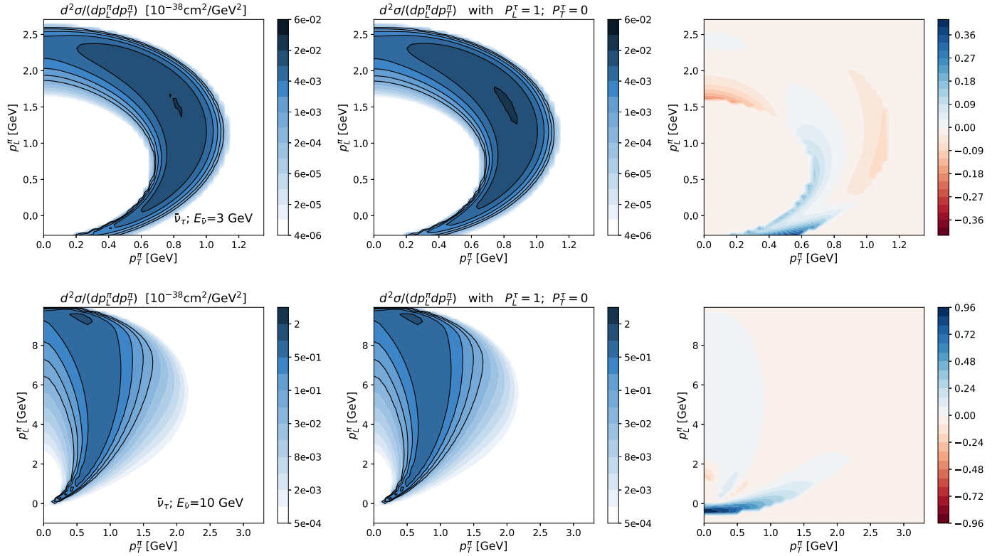
Fig. 3. Same as Fig. 2 but in this case for the anti-neutrino \bar{\nu}_\tau A_Z \rightarrow \tau^+(\pi^+ \nu_\tau)X reaction at only E_\nu = 3 and 10 GeV.
