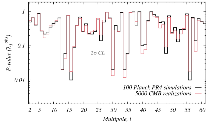
Fig. 3. p -value plot of the smallest eigenvalue of the Power tensor, \lambda_l^{\text{obs}} , for the first sixty multipoles of the CMB map derived using the Planck NPIPE processing pipeline (PR4) and cleaned using the Commander method. The 2\sigma (95%) level is also indicated by a gray horizontal line. The curves correspond to the two different simulation sets used viz., 100 Planck like simulations provided by Planck collaboration and 5000 mock CMB maps based on best fit theoretical power spectrum from Planck derived latest cosmological parameters.
