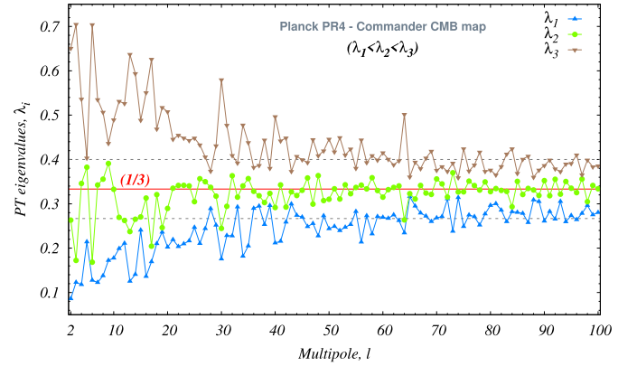
Fig. 1. Eigenvalues of the Power tensor for each ' l ' in the CMB map from Planck PR4 data obtained using Commander method. The horizontal red line is the expectation value of the eigenvalues when isotropy holds viz., \langle \lambda_i \rangle = 1/3 , and the two dashed lines denote the \pm 20\% deviation around this expectation i.e., \pm 1/5^{\text{th}} \times 1/3 = \pm 1/15 .
