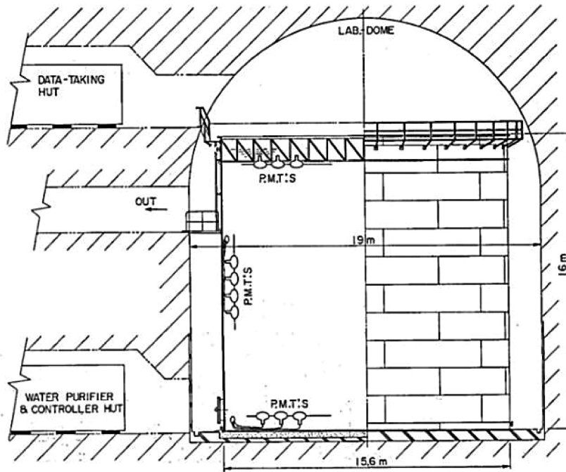
Fig. 13. Original Kamiokande detector.
