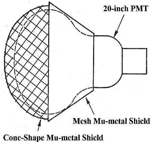
Fig. 10. Magnetic shield for the 20-in PMT.
