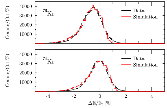
Fig. 2. Measured kinetic-energy distributions of the outgoing ^{74,76}\text{Kr} beams (black) compared to results of detailed GEANT4 simulations (red) performed with UCGRETINA [25] to determine the LH 2 target thickness. Both simulations provided consistent results for the target thickness.
