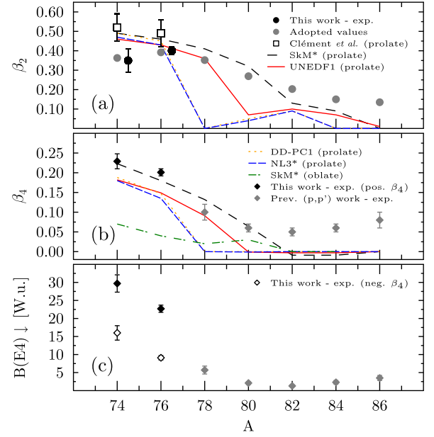
Fig. 3. (a) Experimental \beta_2 values [new data (black circles), adopted values [38,39] (gray circles)], and values determined by Clément et al. for the unperturbed prolate configuration [24] (white squares)], (b) \beta_4 values [new data (black diamonds) and previous (p, p') data [40] (gray diamonds)], and (c) experimental B(E4; 4_1^+ \rightarrow 0_1^+) strengths in neutron-deficient Kr isotopes. Alternative values, obtained for the negative \beta_4 values discussed in the text, are presented with white diamonds in panel (c). Theoretical DFT predictions for the corresponding observables are shown in panels (a) and (b). These were obtained using the energy density functionals SkM* (black longer dashed line) and UNEDF1 (red solid line), as well as two covariant energy density functionals DD-PC1 (orange dotted line) and NL3* (blue short dashed line). For \beta_2 , predictions are shown for the prolate minimum only. In addition, predictions for the oblate minimum made with SkM* are shown (green dotted-dashed line) in (b).
