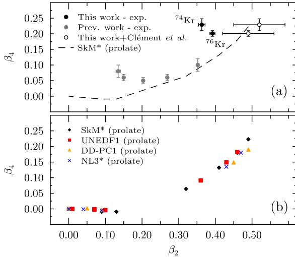
Fig. 4. Hexadecapole deformation parameter \beta_4 plotted against \beta_2 : (a) experimental values; (b) theoretical predictions. Earlier data for \beta_4 are from Ref. [40] (gray circles). The experimental \beta_2 values were taken from Ref. [38,39]. The open circles in (a) correspond to the \beta_2 values calculated from the quadrupole moments Q_{20} of the unperturbed prolate configurations reported in Ref. [24]. The SkM* predictions are marked in panel (a) with a dashed line.
