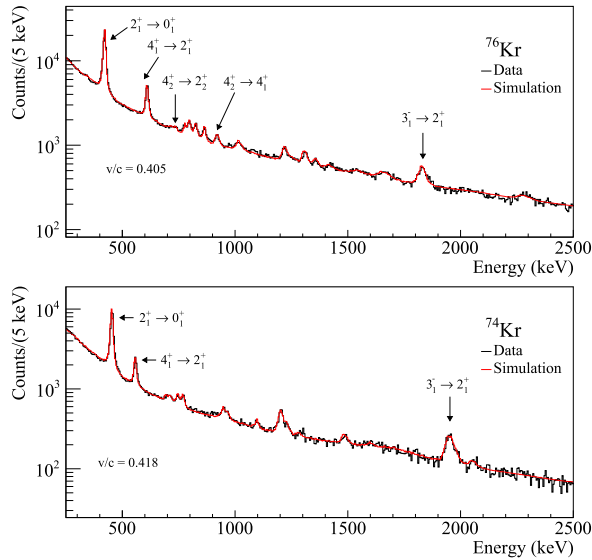
Fig. 1. Doppler-corrected, in-beam \gamma -ray spectra for ^{76}\text{Kr} (top) and ^{74}\text{Kr} (bottom). Data are shown in black. GEANT4 simulations performed with UCGRETINA [25] are presented in red. A prompt background consisting of two exponential functions was included in the simulation. Besides transitions from the J^\pi = 2_1^+ and 3_1^- states, observed transitions of the populated 4^+ states are highlighted.
