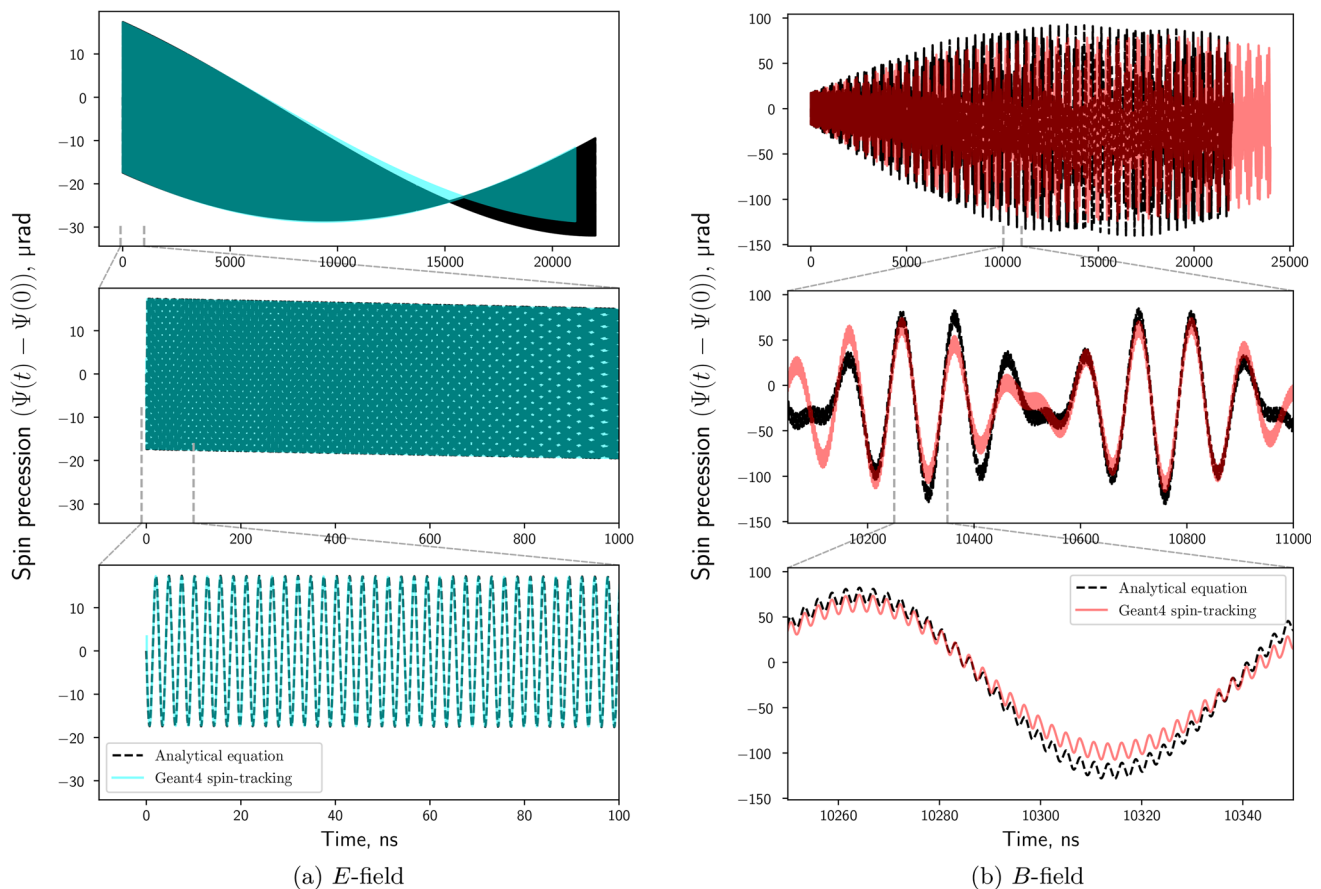
Fig. 11 Accumulation of Berry's phase due to oscillations of the spin around perpendicular axes. a Shows the case of equal oscillation frequencies (resonant oscillations) around the two axes caused by changing E -field in the muon reference frame. b Shows the Berry phase for the
