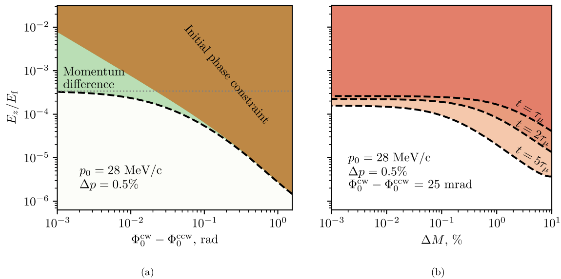
Fig. 5 Limit on the longitudinal E -field, E_z , when considering alternating CW/CCW injections, where the difference in mean momentum averaged over all injected muons for injections of CW and CCW beams is fixed at \Delta p = 0.5\% . a Shows the limit as a function of the initial phase difference \Phi_0^{\text{cw}} - \Phi_0^{\text{ccw}} . The horizontal dashed line indicates the limit coming from \Delta p , keeping all other parameters equal between the two injection modes. The brown area is the constraint coming from the dif-
