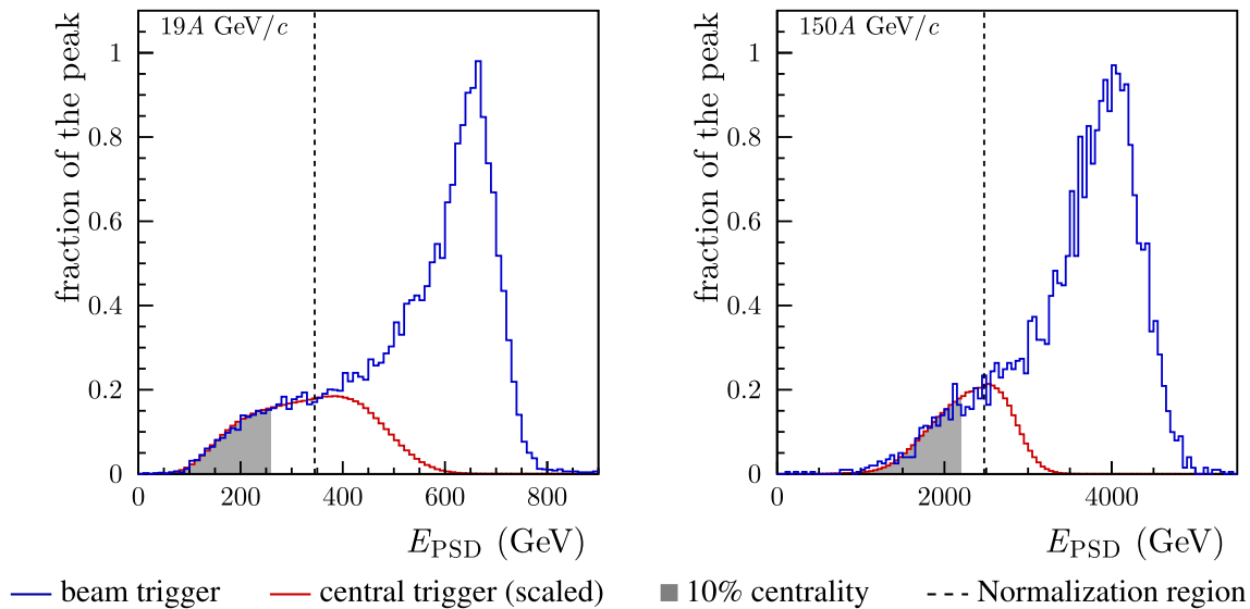
Fig. 3 Distributions of the energy E_{\text{PSD}} measured by the PSD calorimeter for 19A (left plot) and 150A GeV/c (right plot) beam momentum, for minimum-bias selected (blue histograms) and central trigger selected (red histograms) events. Histograms are normalized to
