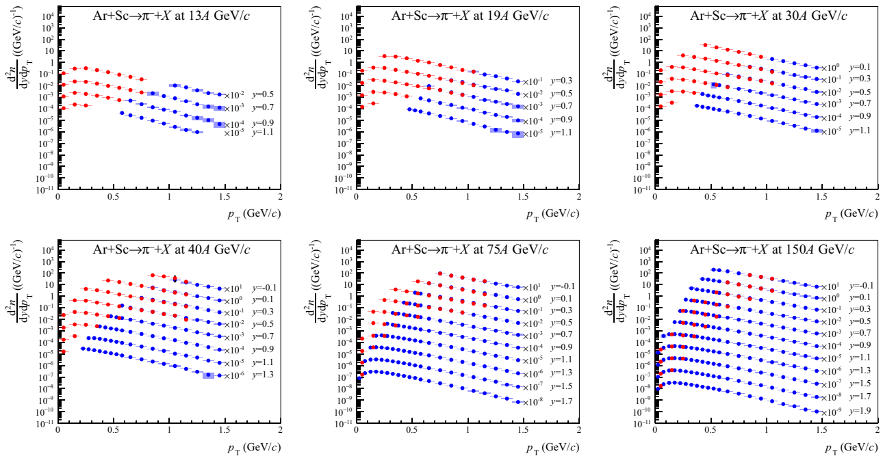
Fig. 60 Comparison of transverse momentum spectra in rapidity slices of \pi^- obtained with dE/dx (blue) and tof - dE/dx (red) methods, produced in 10% most central Ar+Sc collisions at 13A to 150A GeV/c. For graphical presentations, the spectra are multiplied by factors given in
