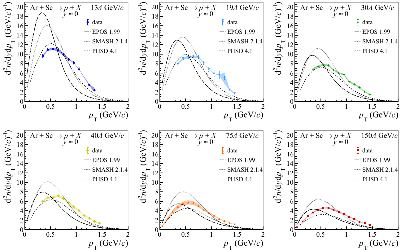
Fig. 48 Transverse momentum distributions of protons at mid-rapidity produced in 10% most central Ar+Sc interactions at 13A, 19A, 30A, 40A, 75A and 150A GeV/c compared with models: EPOS 1.99 [68], PHSD 4.1 [69,70] and SMASH 2.1.4 [71,72]
