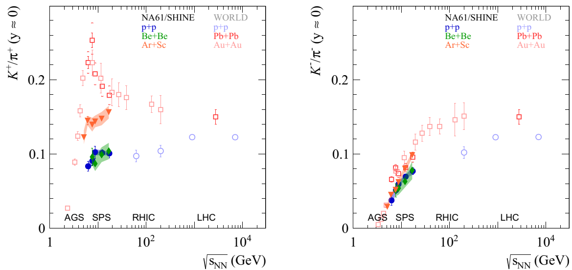
Fig. 33 The energy dependence of the K/\pi ratio at mid-rapidity of positively ( left ) and negatively ( right ) charged particles for central Ar+Sc, Be+Be ([17]), Pb+Pb ([2,3,53–55]) and Au+Au ([4,56–61])
