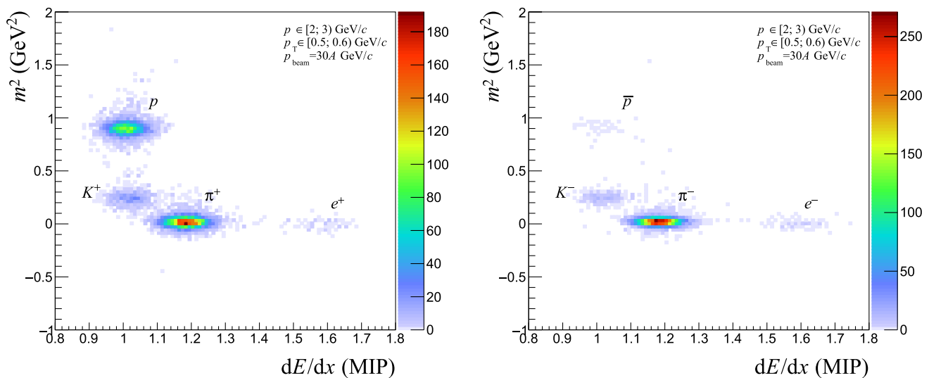
Fig. 10 Example distributions of particles in m^2 and dE/dx plane in a single bin ( 2 \text{ GeV}/c < p < 3 \text{ GeV}/c , 0.5 \text{ GeV}/c < p_T < 0.6 \text{ GeV}/c ) for positively (left) and negatively (right) charged particles measured in central Ar+Sc collisions at 30A GeV/c
