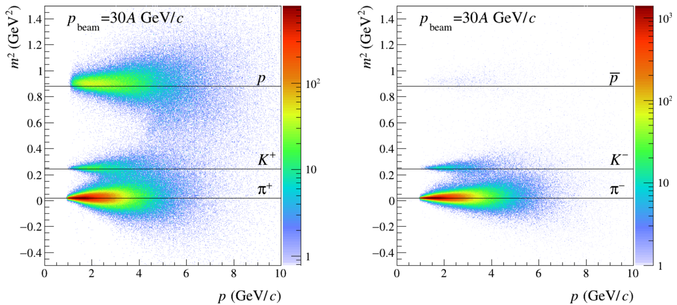
Fig. 9 Distribution of particles in the plane laboratory momentum and mass squared derived using time-of-flight measured by ToF-R ( right ) and ToF-L ( left ) produced in central Ar+Sc collisions at 30A GeV/c. The lines show the expected mass squared values for different hadron species
