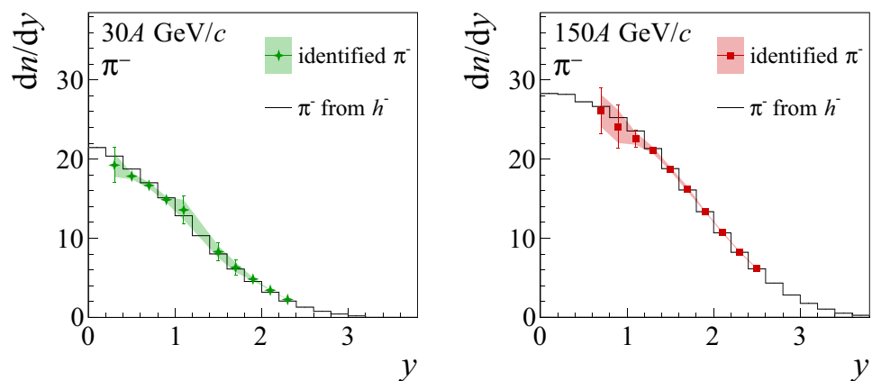
Fig. 22 Comparison of rapidity spectra of negatively charged pions measured with dE/dx and tof-dE/dx methods (colored markers) against the results obtained with the h^- method [17] (black line). Both results consider 10% most central Ar+Sc collisions, and the comparison is displayed for beam momenta of 30A and 150 A GeV/c. The statistical uncertainties do not exceed the size of the markers and the systematic uncertainties are shown as shaded bands
