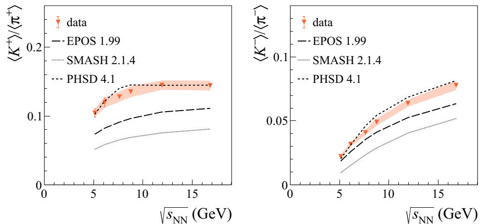
Fig. 47 The ratios of mean multiplicity \langle K^+ \rangle / \langle \pi^+ \rangle and \langle K^- \rangle / \langle \pi^- \rangle produced in 10% most central Ar+Sc interactions at 13A, 19A, 30A, 40A, 75A and 150A GeV/c in dependence on collision energy compared with models: EPOS 1.99 [68], PHSD 4.1 [69,70] and SMASH 2.1.4 [71,72]
