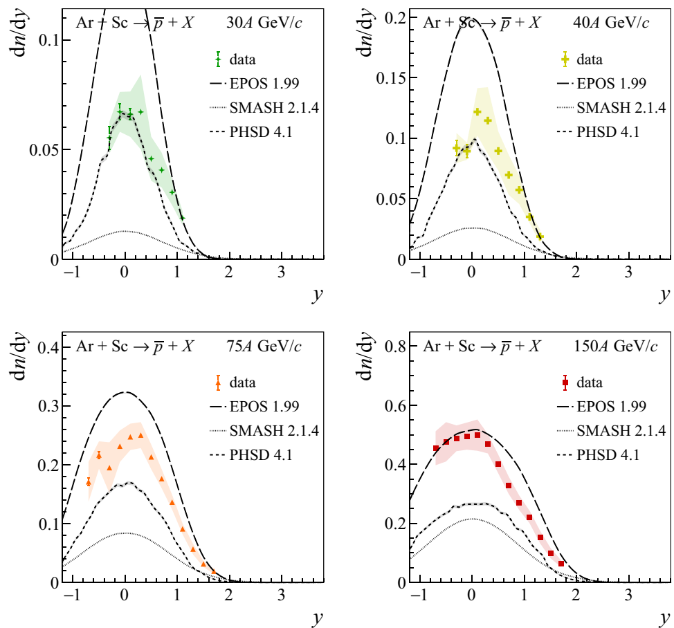
Fig. 51 Rapidity spectra of antiprotons produced in 10% most central Ar+Sc interactions at 30A, 40A, 75A and 150A GeV/c in comparison with models: EPOS 1.99 [68], PHSD 4.1 [69, 70] and SMASH 2.1.4 [71, 72]
