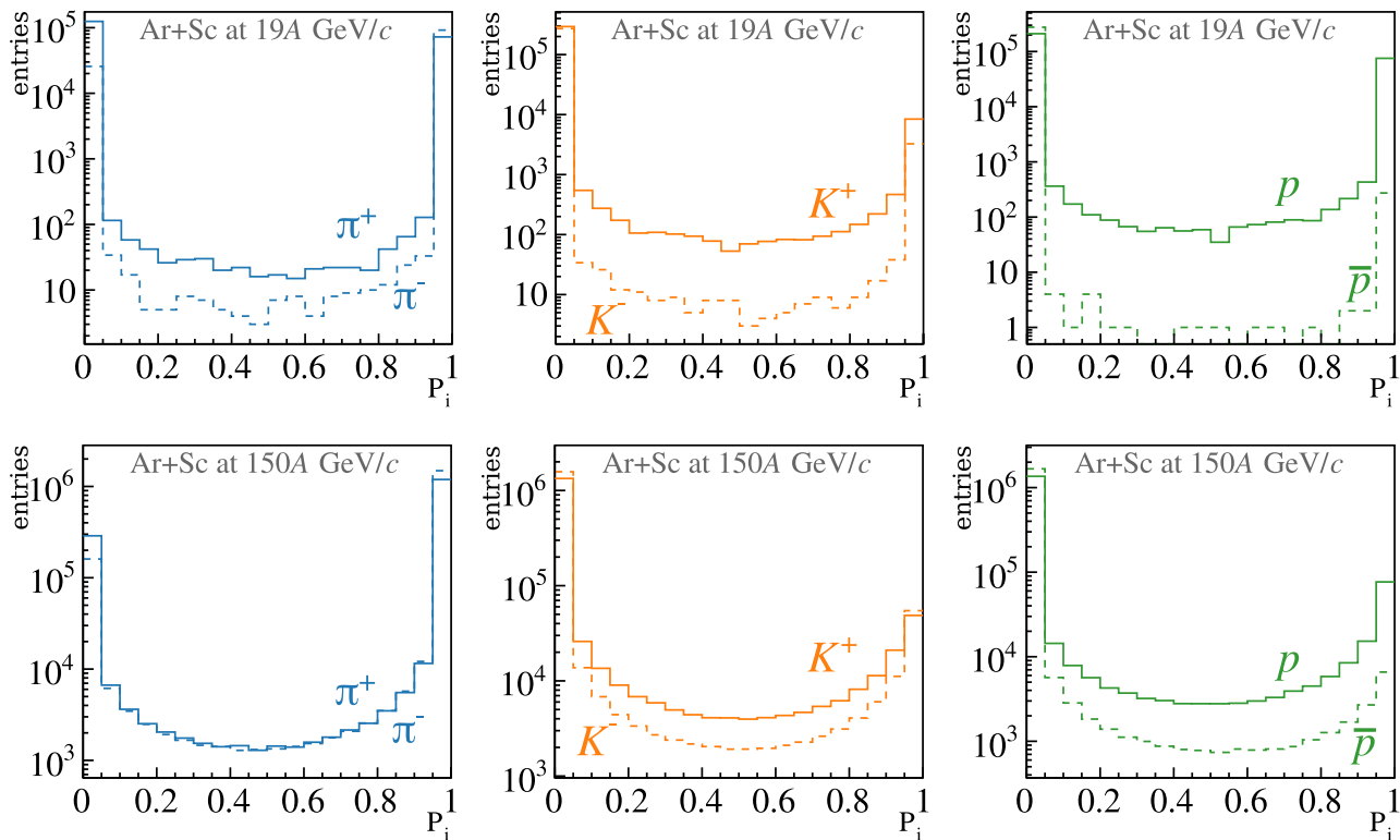
Fig. 13 Distribution of probabilities of a track being a pion, kaon, proton for positively (solid lines) and negatively (dashed lines) charged particles from tof - dE/dx measurements in central Ar+Sc collisions at 19A (top) and 150A GeV/c (bottom)
