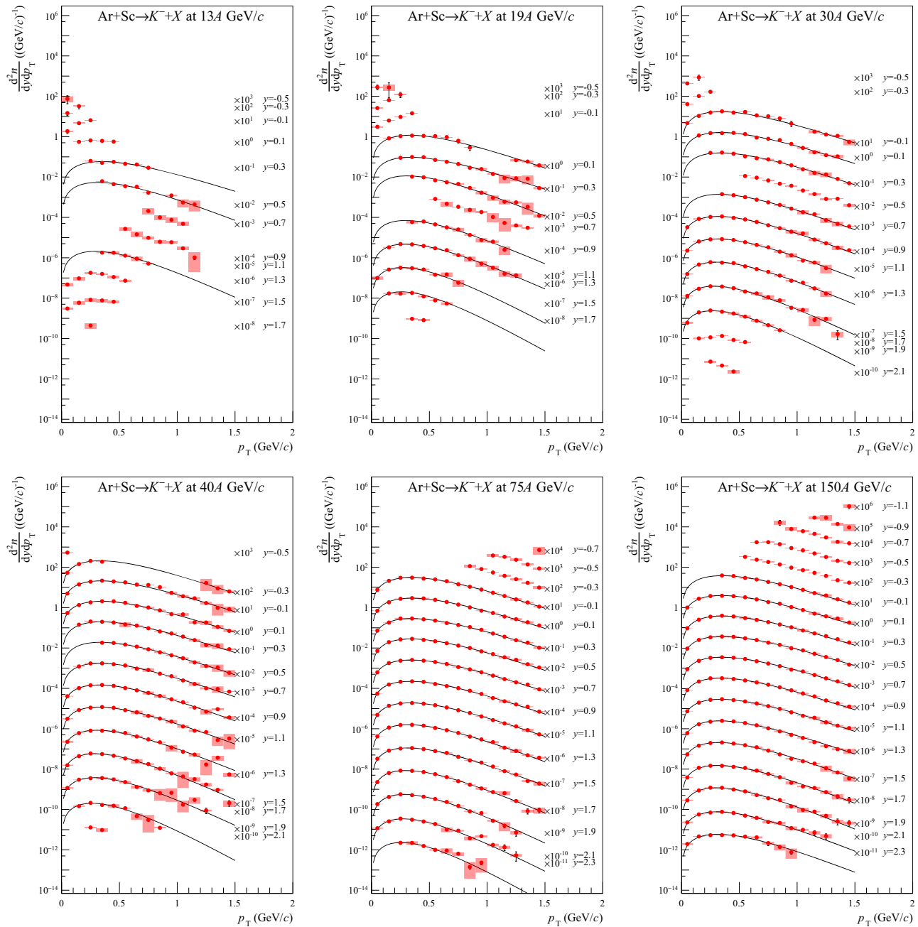
Fig. 56 Transverse momentum spectra in rapidity slices of K^- produced in 10% most central Ar+Sc collisions at 13A to 150A GeV/c. For graphical presentations, the spectra are multiplied by factors given in the plots. Lines correspond to fitted exponential functions (Eq. 18).
