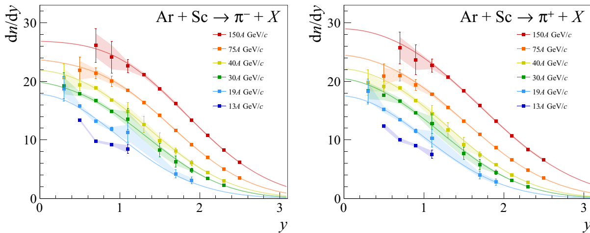
Fig. 20 Rapidity spectra of charged pions ( \pi^+ and \pi^- ) measured with dE/dx and \text{tof-}dE/dx methods in 10% most central Ar+Sc collisions. The line is a sum of two Gaussians, equidistant from mid-rapidity with
