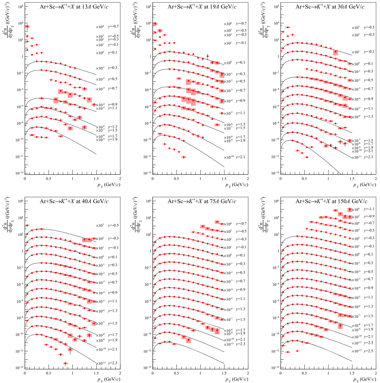
Fig. 55 Transverse momentum spectra in rapidity slices of K^+ produced in 10% most central Ar+Sc collisions at 13A to 150A GeV/c. For graphical presentations, the spectra are multiplied by factors given in the plots. Lines correspond to fitted exponential functions (Eq. 18).
