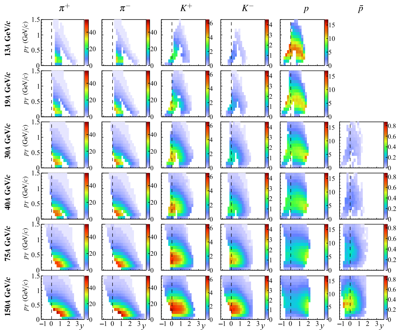
Fig. 16 Two-dimensional distributions ( y vs. p_T ) of double differential yields (Eq. 16) of \pi^- , \pi^+ , K^- , K^+ , p and \bar{p} produced in the 10% most central Ar+Sc interactions at 13A, 19A, 30A, 40A, 75A and 150A GeV/c
