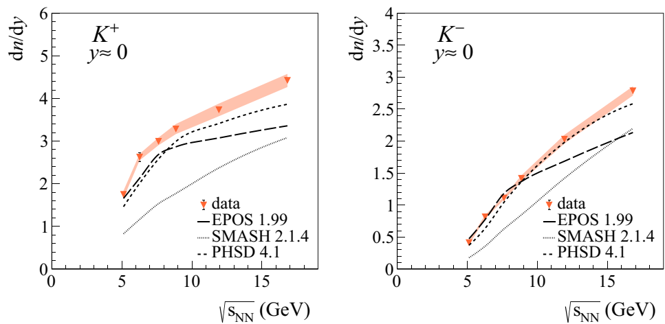
Fig. 42 Mid-rapidity dn/dy yields of K^+ and K^- mesons produced in 10% most central Ar+Sc interactions at 13A, 19A, 30A, 40A, 75A and 150A GeV/c in comparison with models: EPOS 1.99 [68], PHSD 4.1 [69,70] and SMASH 2.1.4 [71,72]
