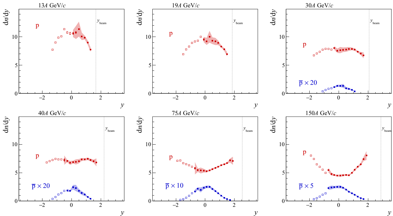
Fig. 29 Rapidity spectra of protons and antiprotons produced in 10% most central Ar+Sc collisions at 13A–150A GeV/c. No data was plotted for anti-protons produced in collisions at p_{\text{beam}} = 13A and 19A GeV/c
