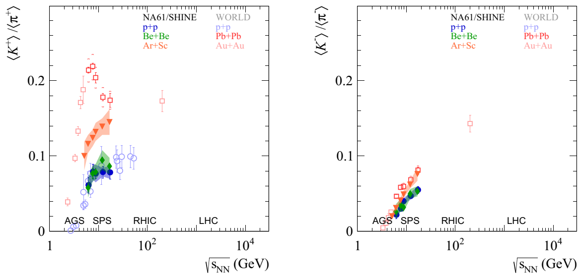
Fig. 34 The energy dependence of the \langle K \rangle / \langle \pi \rangle mean multiplicity ratio of positively ( left ) and negatively ( right ) charged particles for central Ar+Sc, Be+Be ([17]), Pb+Pb ([2,3,53–55]) and Au+Au ([4,56–61])
