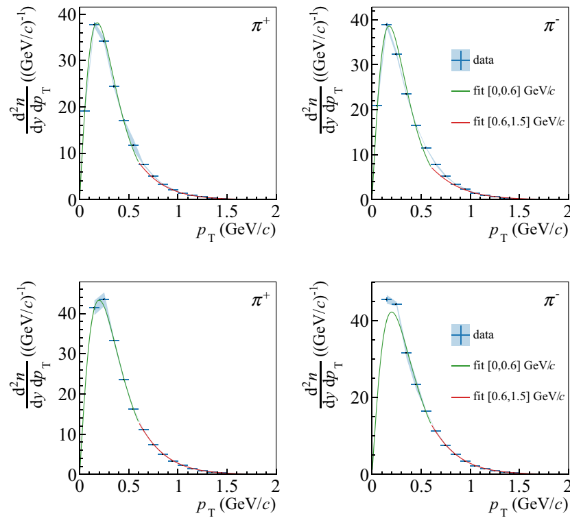
Fig. 19 Example fits to charged pion, \pi^+ (left) and \pi^- (right), transverse momentum spectra ( p_{\text{beam}} = 30A GeV/c and 75A GeV/c at 0.6 < y < 0.8 , top and bottom panels respectively). Exponential fits (Eq. 18) are performed in two regions separately: p_T \in [0.0, 0.6] and p_T \in [0.6, 1.5] GeV/c. The fitted functions are used to extrapolate the yields beyond p_T = 1.5 GeV/c and interpolate the yields in case a gap
