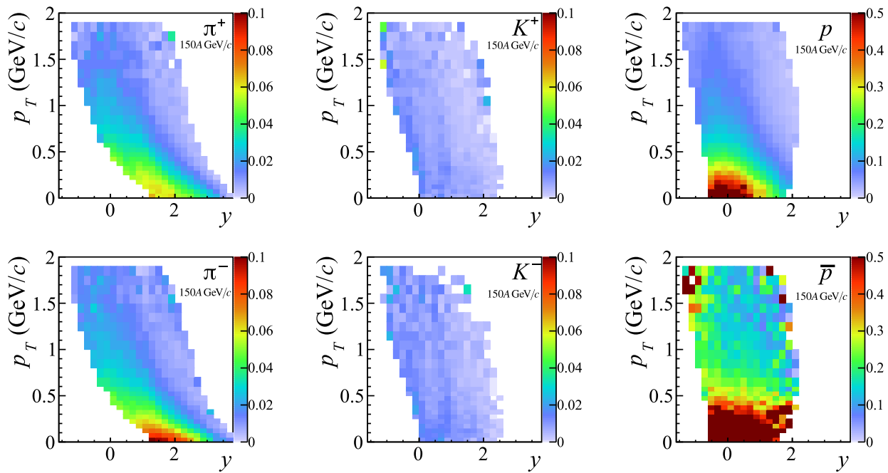
Fig. 15 An example of the relative contribution of weak decay products in spectra of hadrons identified with dE/dx method at 150A GeV/c plotted in y - p_T plane. The corrections are based on the EPOS model with data-derived tuning (see text for details). The feed-down for \pi^- and \pi^+ is typically on the level of 1%-3%, reaching up to 10% in the case of low- p_T \pi^- . Secondary kaons can only originate from sparsely pro-
