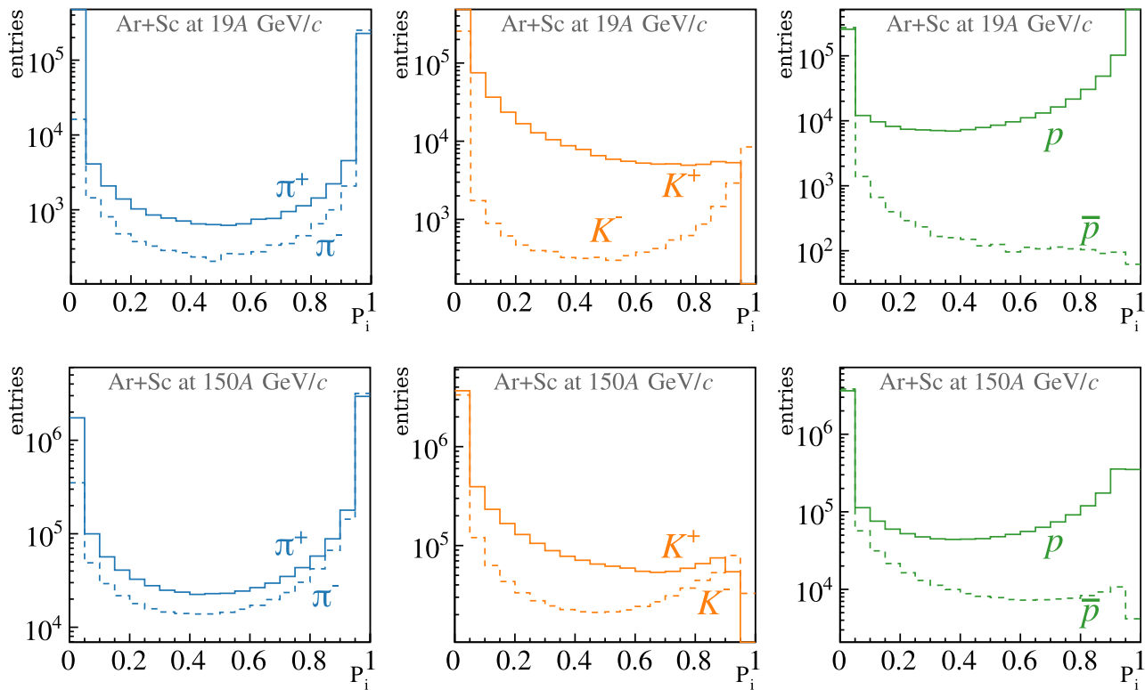
Fig. 12 Distribution of probabilities of a track being a pion, kaon, proton for positively (solid lines) and negatively (dashed lines) charged particles from dE/dx measurements in central Ar+Sc collisions at 19A (top) and 150A GeV/c (bottom)
