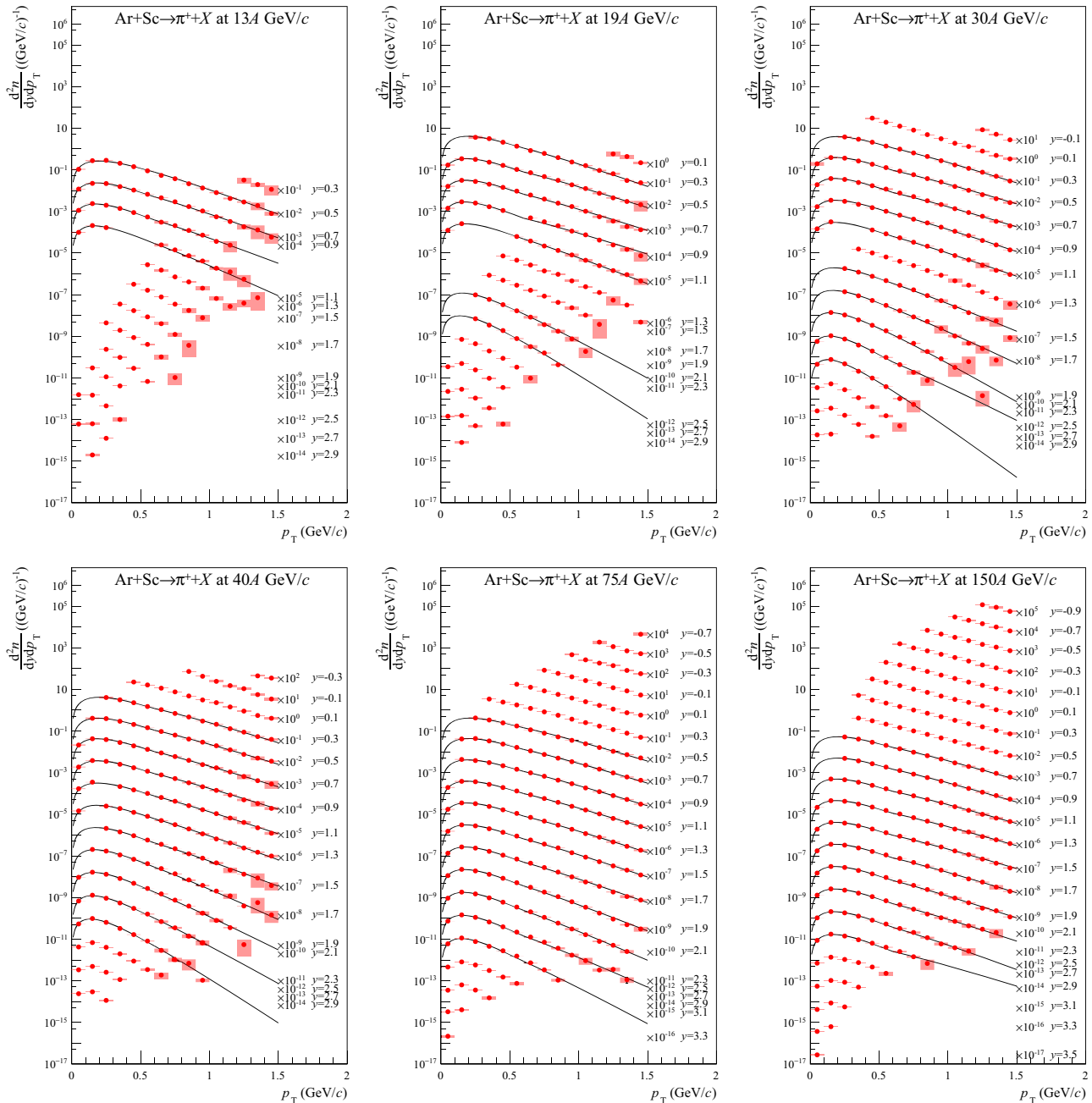
Fig. 53 Transverse momentum spectra in rapidity slices of \pi^+ produced in 10% most central Ar+Sc collisions at 13A to 150A GeV/c. For graphical presentations, the spectra are multiplied by factors given in the plots. Rapidity values given in the legends correspond to the middle of
