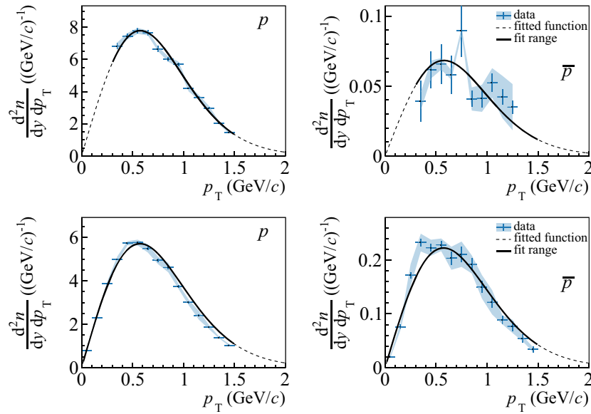
Fig. 28 Example fits to transverse momentum spectra of protons and anti-protons in 10% most central Ar+Sc collisions ( top : p_{\text{beam}} = 30A GeV/c at -0.2 < y < 0.0 and bottom : p_{\text{beam}} = 150A GeV/c at 1.0 < y < 1.2 ). The fitted functions are used to extrapolate the yields beyond p_T = 1.5 GeV/c and interpolate the yields in case a gap in acceptance appears due to the different coverage of the PID methods.
