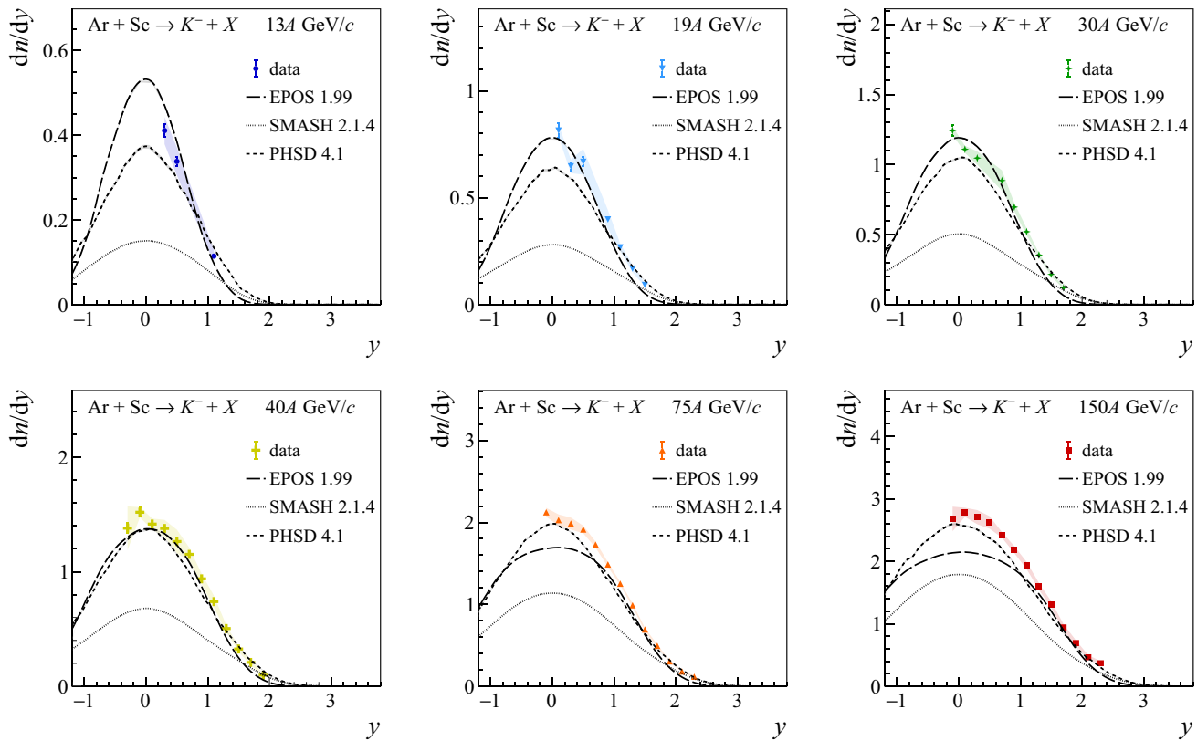
Fig. 44 Rapidity spectra of K^- mesons produced in 10% most central Ar+Sc interactions at 13A, 19A, 30A, 40A, 75A and 150A GeV/c in comparison with models: EPOS 1.99 [68], PHSD 4.1 [69,70] and SMASH 2.1.4 [71,72]
