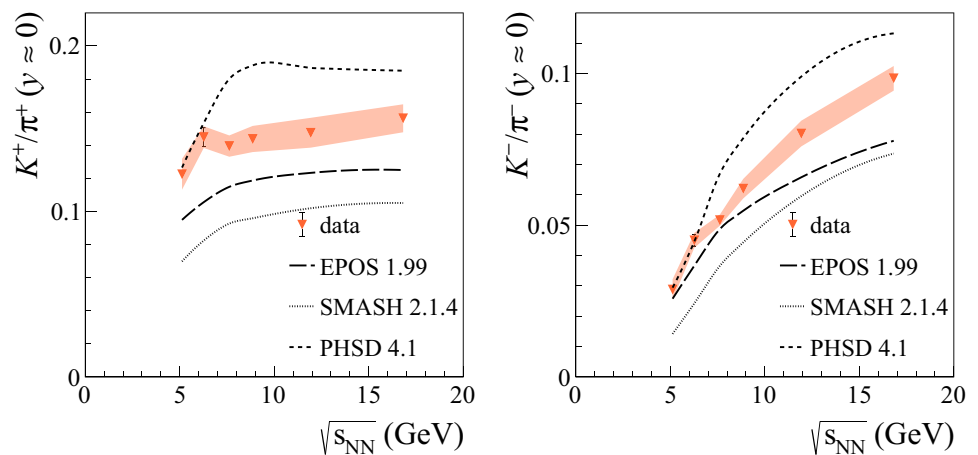
Fig. 46 The ratios of dn/dy yields at mid-rapidity K^+/\pi^+ and K^-/\pi^- produced in 10% most central Ar+Sc interactions at 13A, 19A, 30A, 40A, 75A and 150A GeV/c plotted in dependence on collision energy compared with models: EPOS 1.99 [68], PHSD 4.1 [69,70] and SMASH 2.1.4 [71,72]
