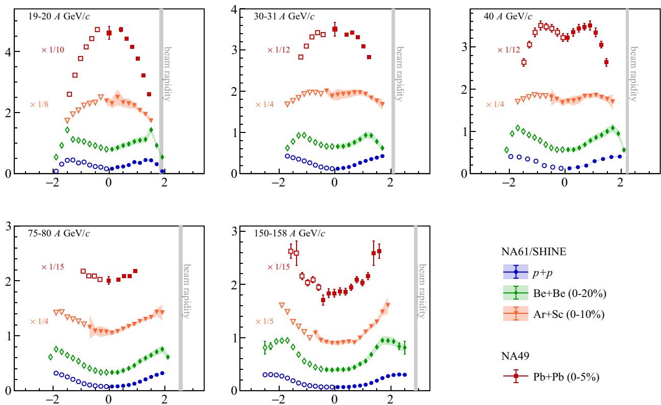
Fig. 35 Proton rapidity spectra in 10% most central Ar+Sc collisions in comparison with other systems: p+p , central Be+Be and central Pb+Pb at five corresponding collision energies. Full markers denote the experimental points, while open ones plot their reflections with respect
