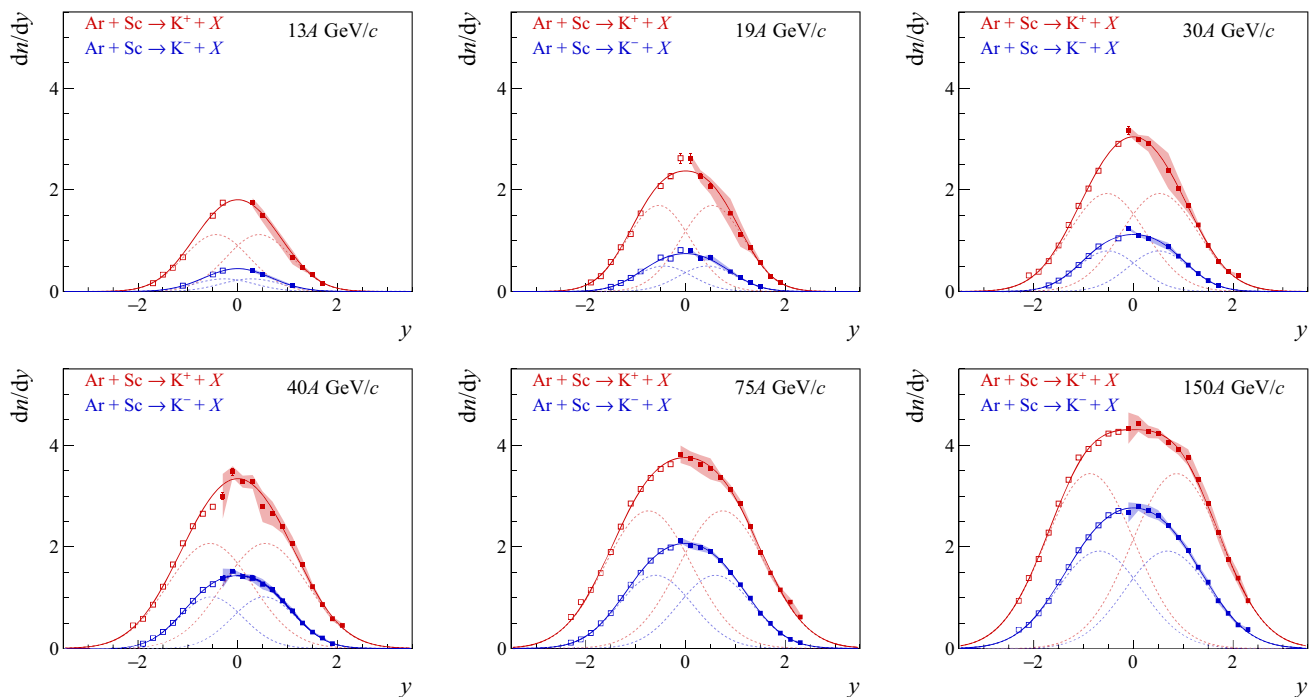
Fig. 26 Rapidity distributions of K^+ and K^- in 10% most central Ar+Sc collision at 13A–150A GeV/c beam momenta. Data points are plotted along with double-Gaussian fits (Eq. 19). The vertical bars rep-
