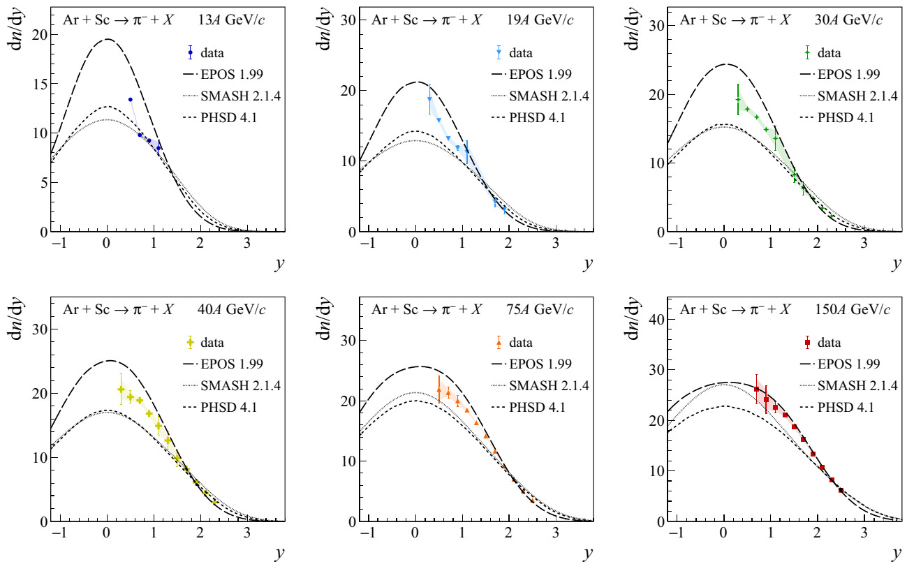
Fig. 37 Rapidity spectra of \pi^- mesons produced in 10% most central Ar+Sc interactions at 13A, 19A, 30A, 40A, 75A and 150A GeV/c in comparison with models: EPOS 1.99 [68], PHSD 4.1 [69,70] and SMASH 2.1.4 [71,72]
