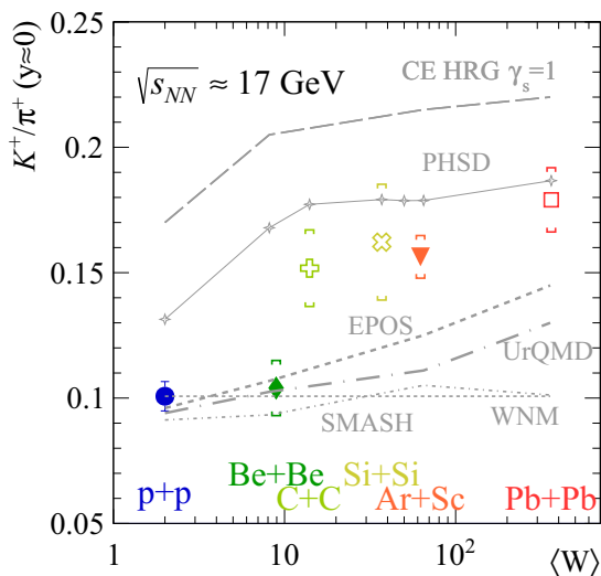
Fig. 52 System size dependence of the K^+/\pi^+ ratio (at y \approx 0 ) in central nucleus-nucleus and inelastic p+p interactions obtained at beam momenta of \approx 150 A GeV/c ( \sqrt{s_{NN}} \approx 17 GeV) compared with dynamical (EPOS 1.99 [68], PHSD 4.1 [69, 70] and UrQMD [75, 76]) and statistical (HRG [77]) models. Additionally, WNM [25] prediction is shown as a horizontal dashed line
