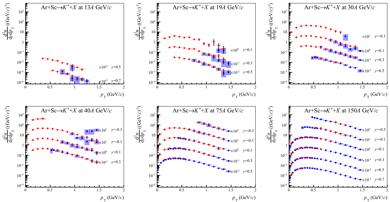
Fig. 61 Comparison of transverse momentum spectra in rapidity slices of K^+ obtained with dE/dx (blue) and tof - dE/dx (red) methods, produced in 10% most central Ar+Sc collisions at 13A to 150A GeV/c. For graphical presentations, the spectra are multiplied by factors given in
