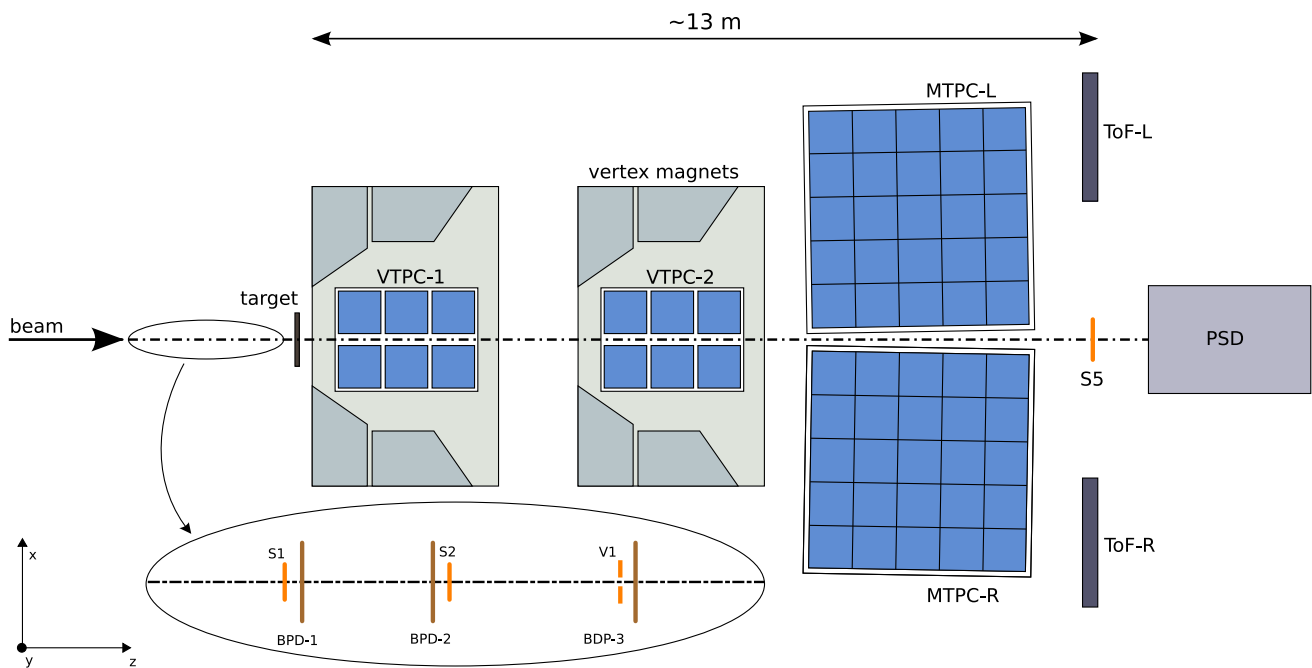
Fig. 1 The schematic layout of the NA61/SHINE experiment at the CERN SPS [18] showing the components used for the Ar+Sc energy scan. The beam instrumentation is sketched in the inset. The alignment of the chosen coordinate system as shown in the figure. The nominal
