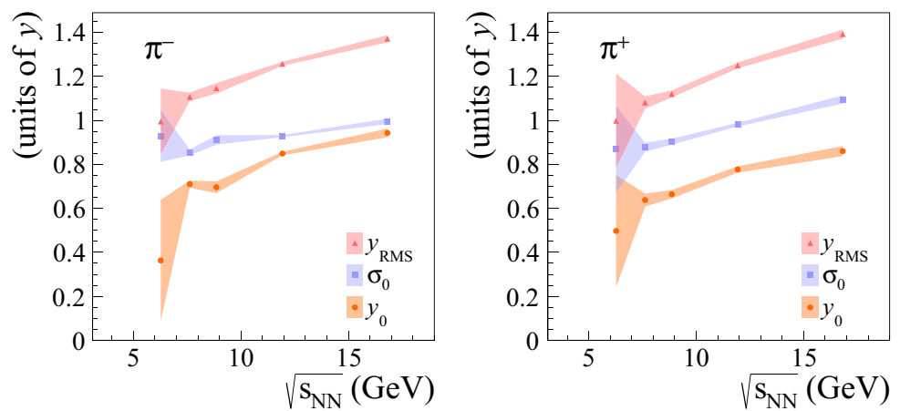
Fig. 21 The parameters of double-Gaussian fit (Eqs. 19 and 20) to charged pion rapidity spectra in 10% most central Ar+Sc collisions. The shaded bands illustrate the statistical uncertainties of the fit
