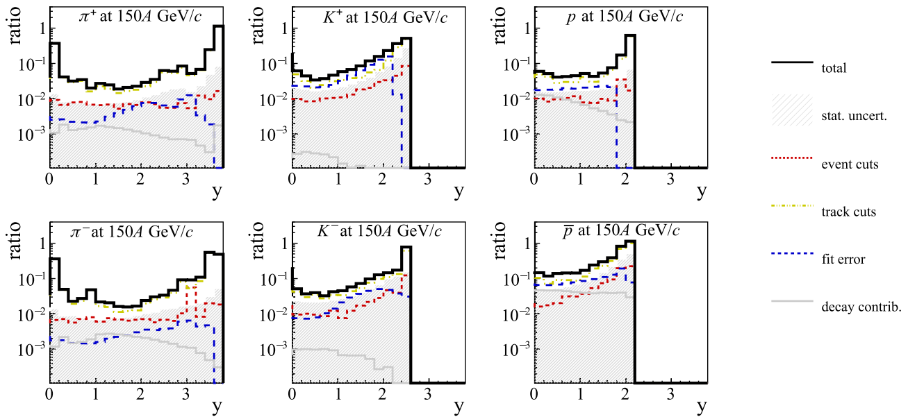
Fig. 17 Systematic uncertainty relative to the measured yield of double-differential distributions obtained with dE/dx PID method, integrated in p_T , shown for each identified species in dependence on rapidity y at p_{\text{beam}} = 150A GeV/c. Different contributions to the total
