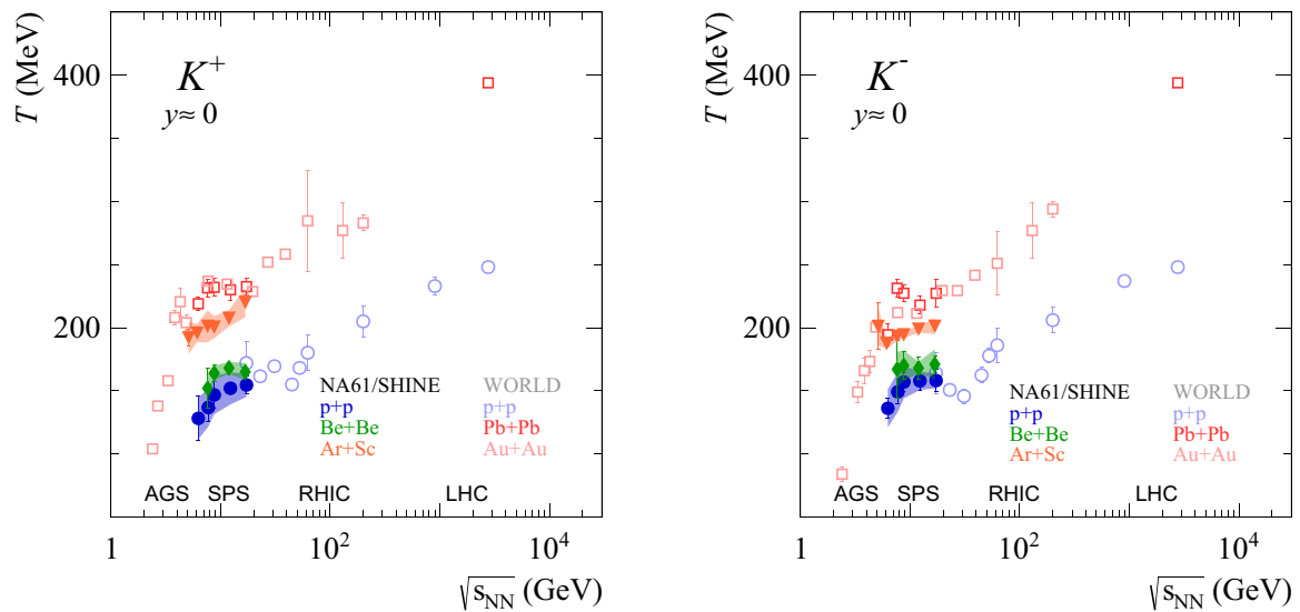
Fig. 32 The energy dependence of the inverse slope parameter T of p_T spectra at mid-rapidity of positively ( left ) and negatively ( right ) charged K mesons for central Ar+Sc, Be+Be ([17]), Pb+Pb ([2,3,53–55]) and
