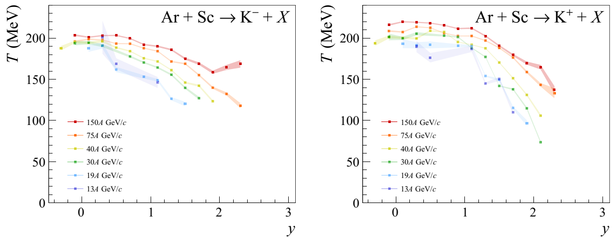
Fig. 24 Rapidity dependence of the inverse slope parameter T fitted to charged kaon p_T distribution in 10% most central Ar+Sc collisions. The shaded bands illustrate the statistical uncertainties of the fit
