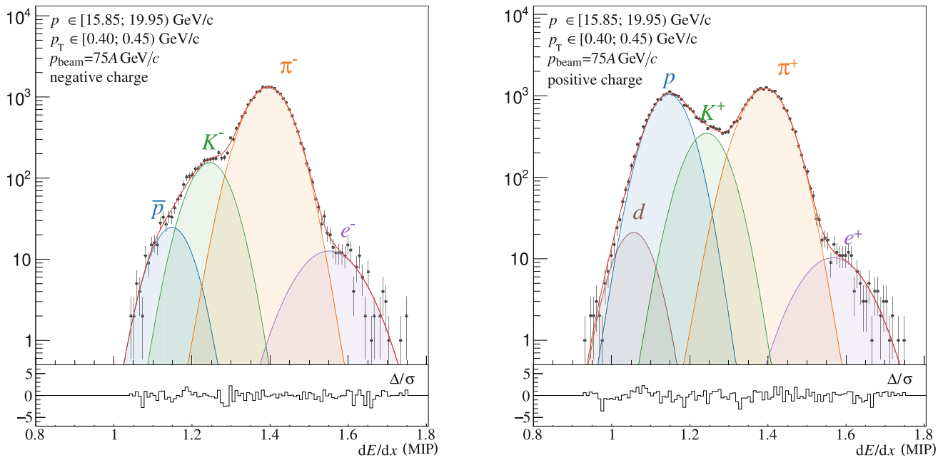
Fig. 8 The dE/dx distributions for negatively ( left ) and positively ( right ) charged particles in a selected p - p_T bin produced in central Ar+Sc collisions at 75A GeV/c. The fits by a sum of contributions
