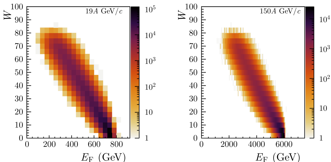
Fig. 4 Distributions of number of wounded nucleons as a function of E_F for all inelastic Ar+Sc collisions at 19A and 150A GeV/c beam momentum calculated from EPOS [26]
