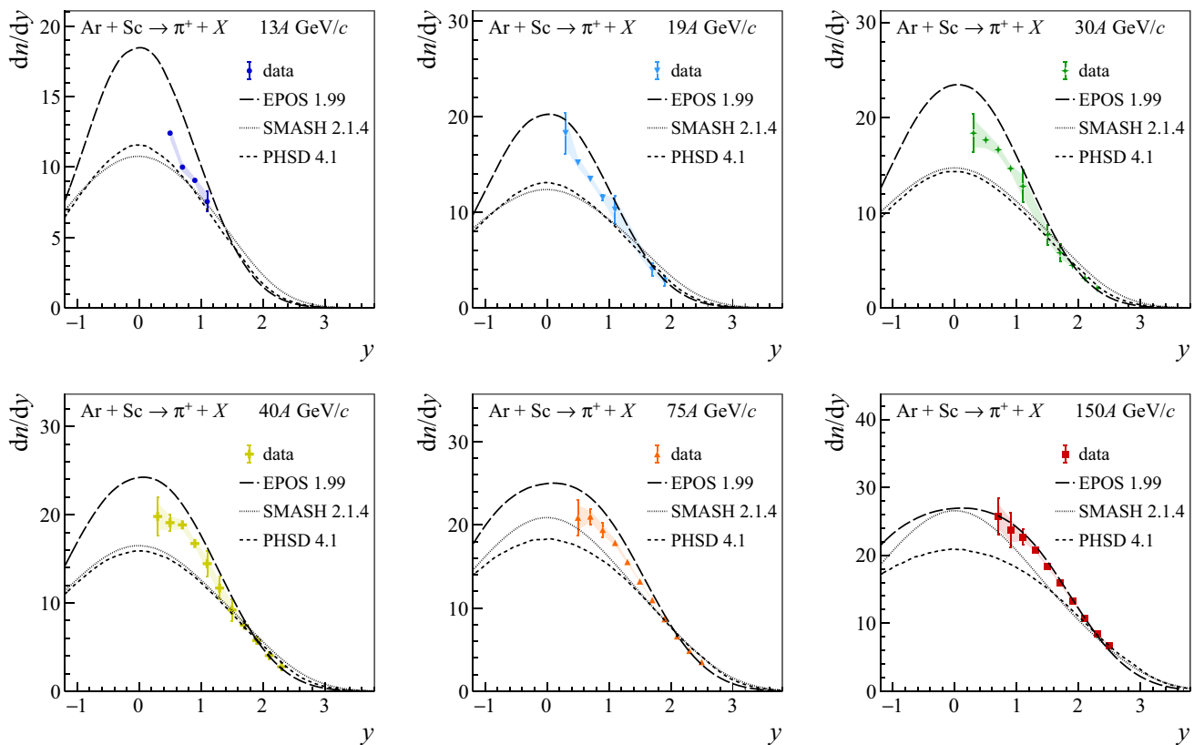
Fig. 36 Rapidity spectra of \pi^+ mesons produced in 10% most central Ar+Sc interactions at 13A, 19A, 30A, 40A, 75A and 150A GeV/c in comparison with models: EPOS 1.99 [68], PHSD 4.1 [69,70] and SMASH 2.1.4 [71,72]
