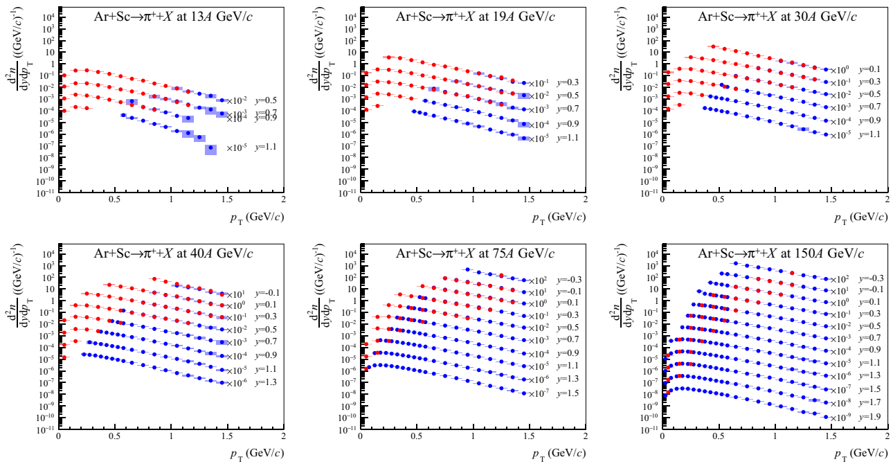
Fig. 59 Comparison of transverse momentum spectra in rapidity slices of \pi^+ obtained with dE/dx (blue) and tof - dE/dx (red) methods, produced in 10% most central Ar+Sc collisions at 13A to 150A GeV/c. For graphical presentations, the spectra are multiplied by factors given in
