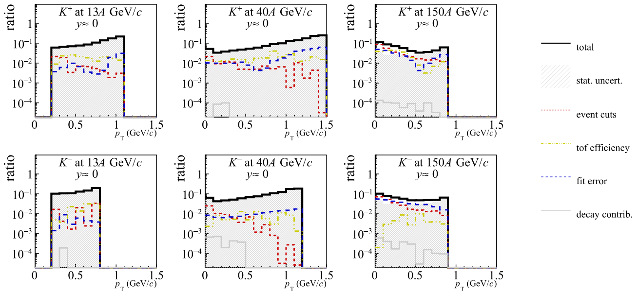
Fig. 18 Systematic uncertainty relative to the measured yield of double-differential distributions in y and p_T for charged kaons, obtained with tof-dE/dx PID method, shown in dependence on transverse
