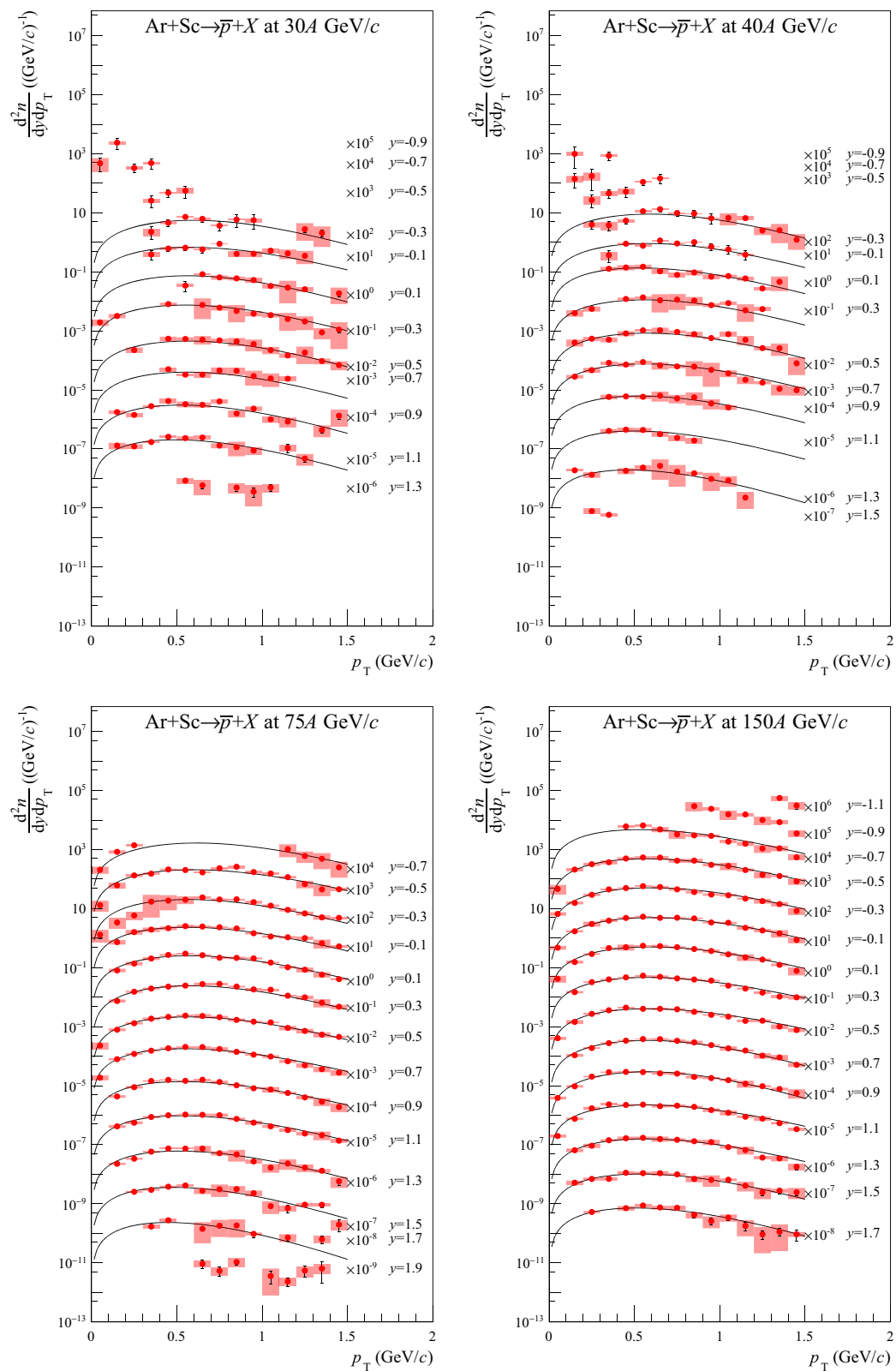
Fig. 58 Transverse momentum spectra in rapidity slices of \bar{p} produced in 10% most central Ar+Sc collisions at 30A to 150A GeV/c. For graphical presentations, the spectra are multiplied by factors given in the plots. Rapidity values given in the legends correspond to the middle of
