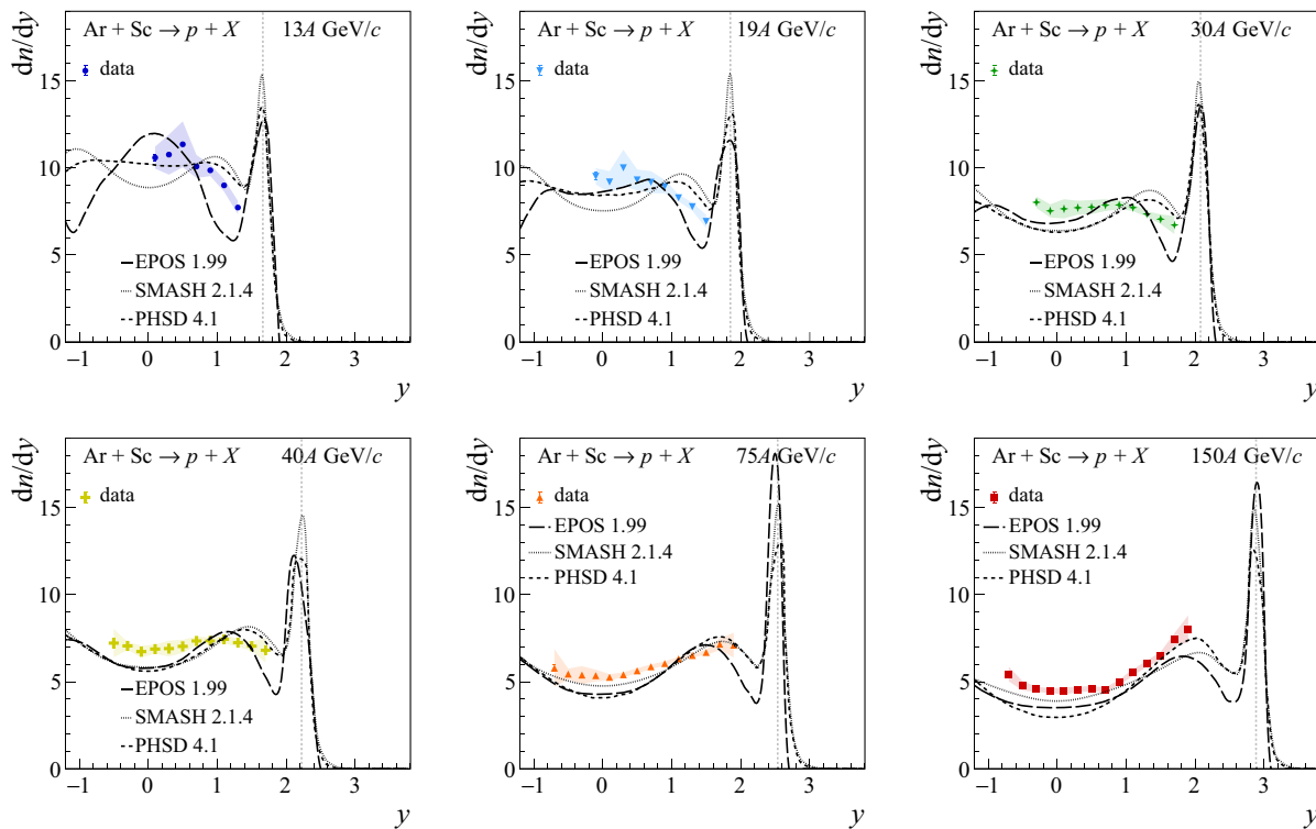
Fig. 50 Rapidity spectra of protons produced in 10% most central Ar+Sc interactions at 13A, 19A, 30A, 40A, 75A and 150A GeV/c in comparison with models: EPOS 1.99 [68], PHSD 4.1 [69,70] and SMASH 2.1.4 [71,72]
