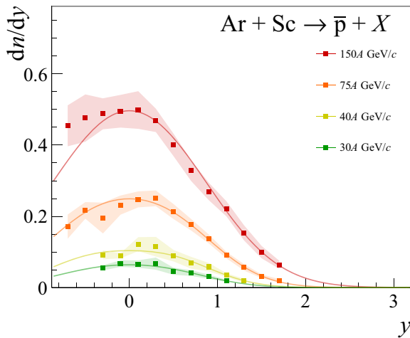
Fig. 31 Rapidity distributions of anti-protons measured in 10% most central Ar+Sc collisions at 30A–150A GeV/c beam momenta. Data points are plotted along with double-Gaussian fits (Eq. 19). Error bars show statistical uncertainties, while shaded bands correspond to systematic uncertainties
