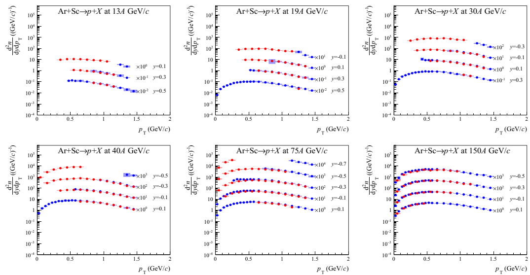
Fig. 63 Comparison of transverse momentum spectra in rapidity slices of p obtained with dE/dx (blue) and tof - dE/dx (red) methods, produced in 10% most central Ar+Sc collisions at 13A to 150A GeV/c. For graphical presentations, the spectra are multiplied by factors given in
