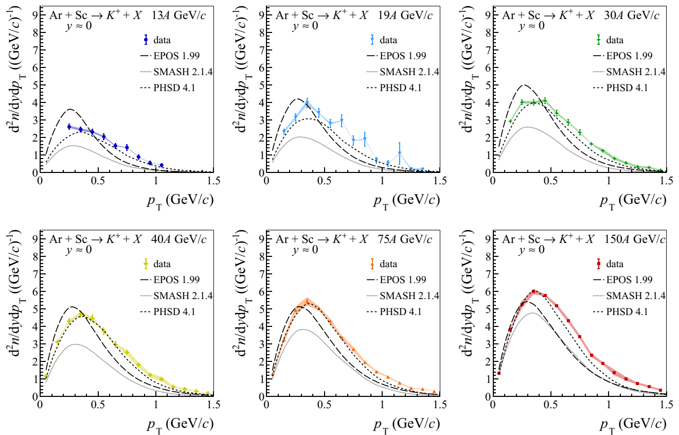
Fig. 39 Mid-rapidity transverse momentum spectra of K^+ mesons produced in 10% most central Ar+Sc interactions at 13A, 19A, 30A, 40A, 75A and 150A GeV/c in comparison with models: EPOS 1.99 [68], PHSD 4.1 [69, 70] and SMASH 2.1.4 [71, 72]
