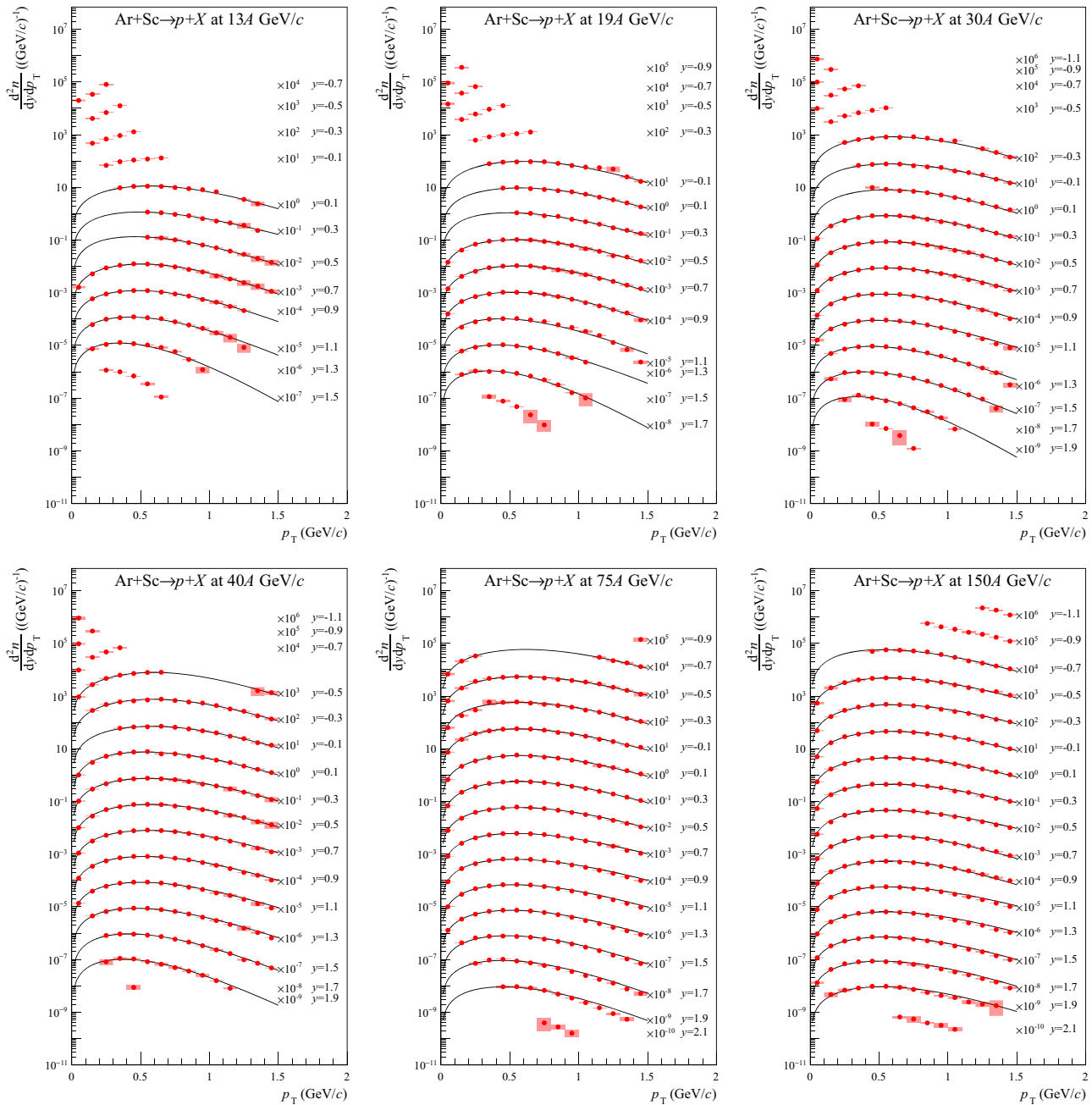
Fig. 57 Transverse momentum spectra in rapidity slices of p produced in 10% most central Ar+Sc collisions at 13A to 150A GeV/c. For graphical presentations, the spectra are multiplied by factors given in the plots. Lines correspond to fitted exponential functions (Eq. 18). Rapidity val-
