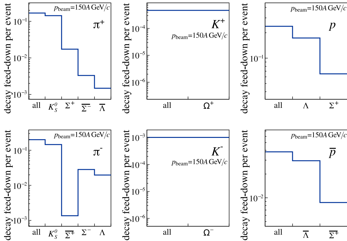
Fig. 14 Contribution per event of reconstructed secondary tracks in the fiducial volume of the detector originating from weak decays and erroneously identified as products of primary interaction (based on EPOS at 150A GeV/c)
