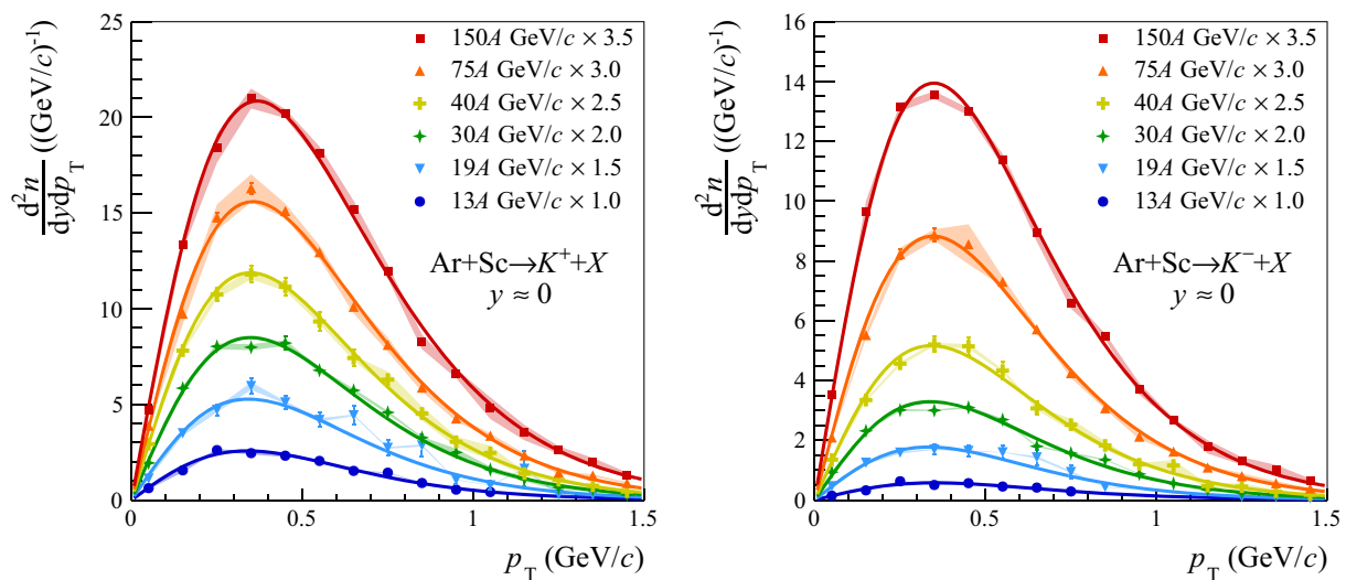
Fig. 25 Transverse momentum spectra of K^+ (left) and K^- (right) at mid-rapidity produced in 10% most central Ar+Sc collisions. Error bars show statistical uncertainties, while shaded bands correspond to systematic uncertainties. The lines represent the fitted functions. The spectra were scaled for better readability
