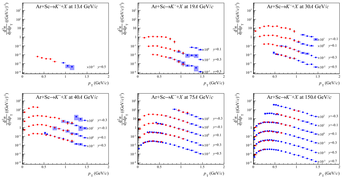
Fig. 62 Comparison of transverse momentum spectra in rapidity slices of K^- obtained with dE/dx (blue) and tof - dE/dx (red) methods, produced in 10% most central Ar+Sc collisions at 13A to 150A GeV/c. For graphical presentations, the spectra are multiplied by factors given in
