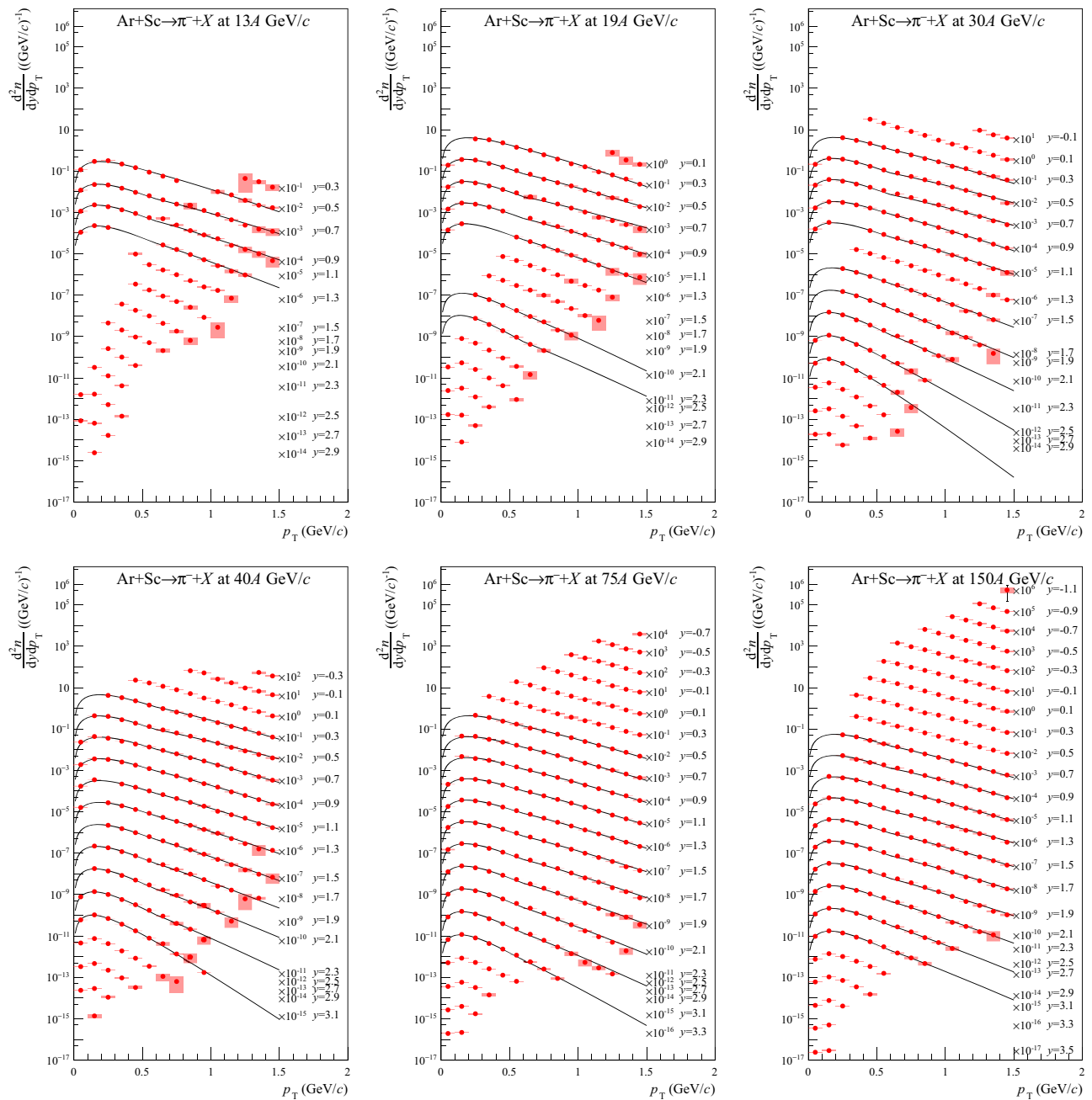
Fig. 54 Transverse momentum spectra in rapidity slices of \pi^- produced in 10% most central Ar+Sc collisions at 13A to 150A GeV/c. For graphical presentations, the spectra are multiplied by factors given in the plots. Rapidity values given in the legends correspond to the middle of
