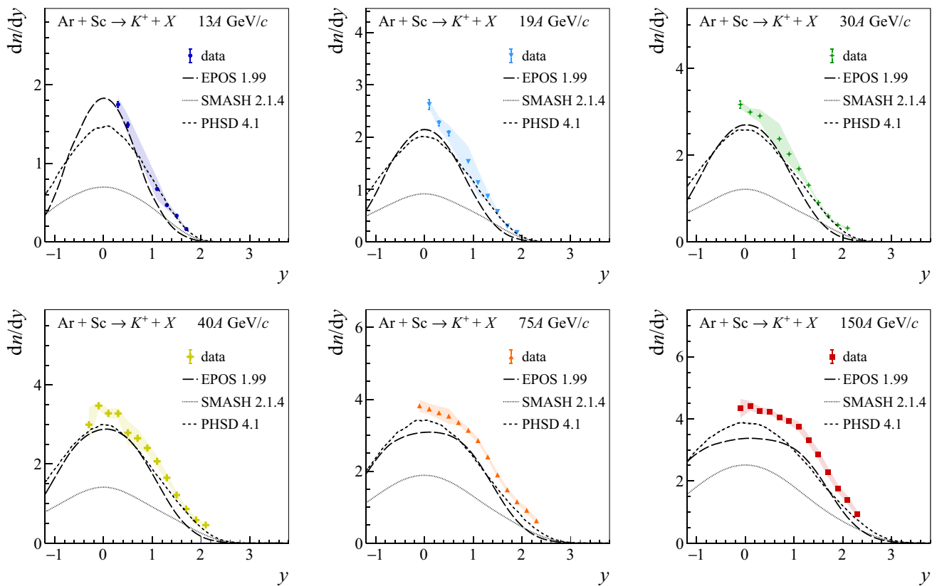
Fig. 43 Rapidity spectra of K^+ mesons produced in 10% most central Ar+Sc interactions at 13A, 19A, 30A, 40A, 75A and 150A GeV/c in comparison with models: EPOS 1.99 [68], PHSD 4.1 [69,70] and SMASH 2.1.4 [71,72]
