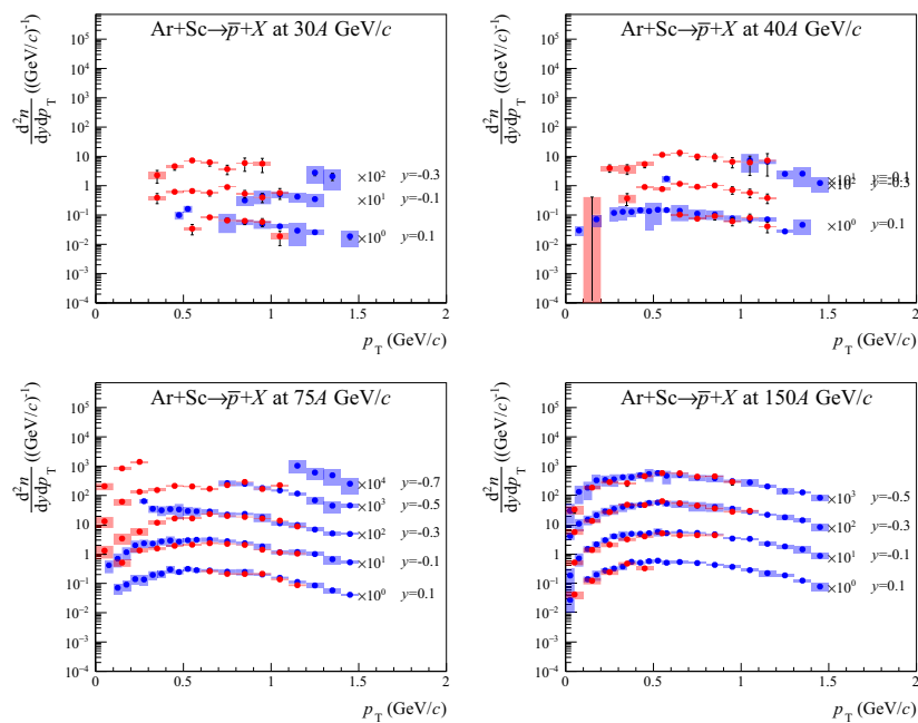
Fig. 64 Comparison of transverse momentum spectra in rapidity slices of \bar{p} obtained with dE/dx (blue) and tof - dE/dx (red) methods, produced in 10% most central Ar+Sc collisions at 30A to 150A GeV/c. For graphical presentations, the spectra are multiplied by factors given in
