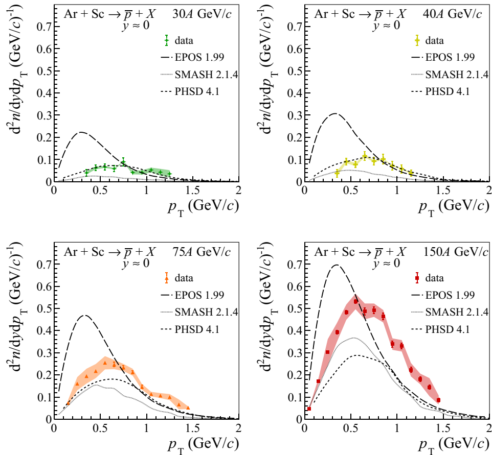
Fig. 49 Transverse momentum distributions of antiprotons at mid-rapidity produced in 10% most central Ar+Sc interactions at 30A, 40A, 75A and 150A GeV/c compared with models: EPOS 1.99 [68], PHSD 4.1 [69,70] and SMASH 2.1.4 [71,72]
