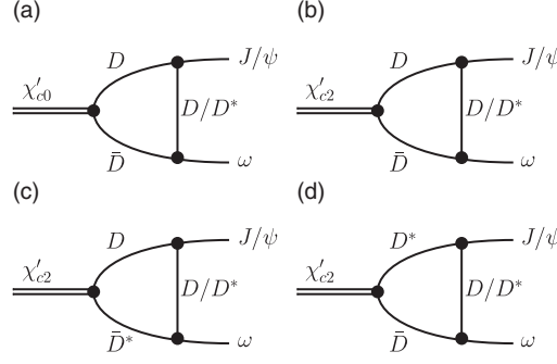
Fig. 1. Typical diagrams describing the X(3915) \rightarrow J/\psi\omega (a) and Z(3930) \rightarrow J/\psi\omega ((b)–(d)) decays. After making the charge conjugate transformation ( D^{(*)} \leftrightarrow \bar{D}^{(*)} ) and the isospin transformation ( D^{(*)0} \leftrightarrow D^{(*)+} and \bar{D}^{(*)0} \leftrightarrow \bar{D}^{(*)-} ), one gets other diagrams.
